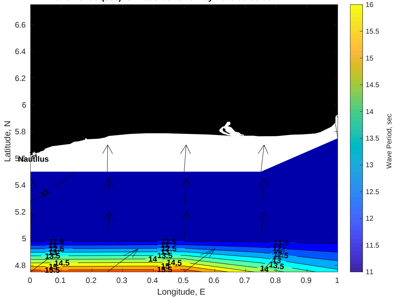
Wave Period (sec) for Nautilus at 26-May-2025 09:00:00
