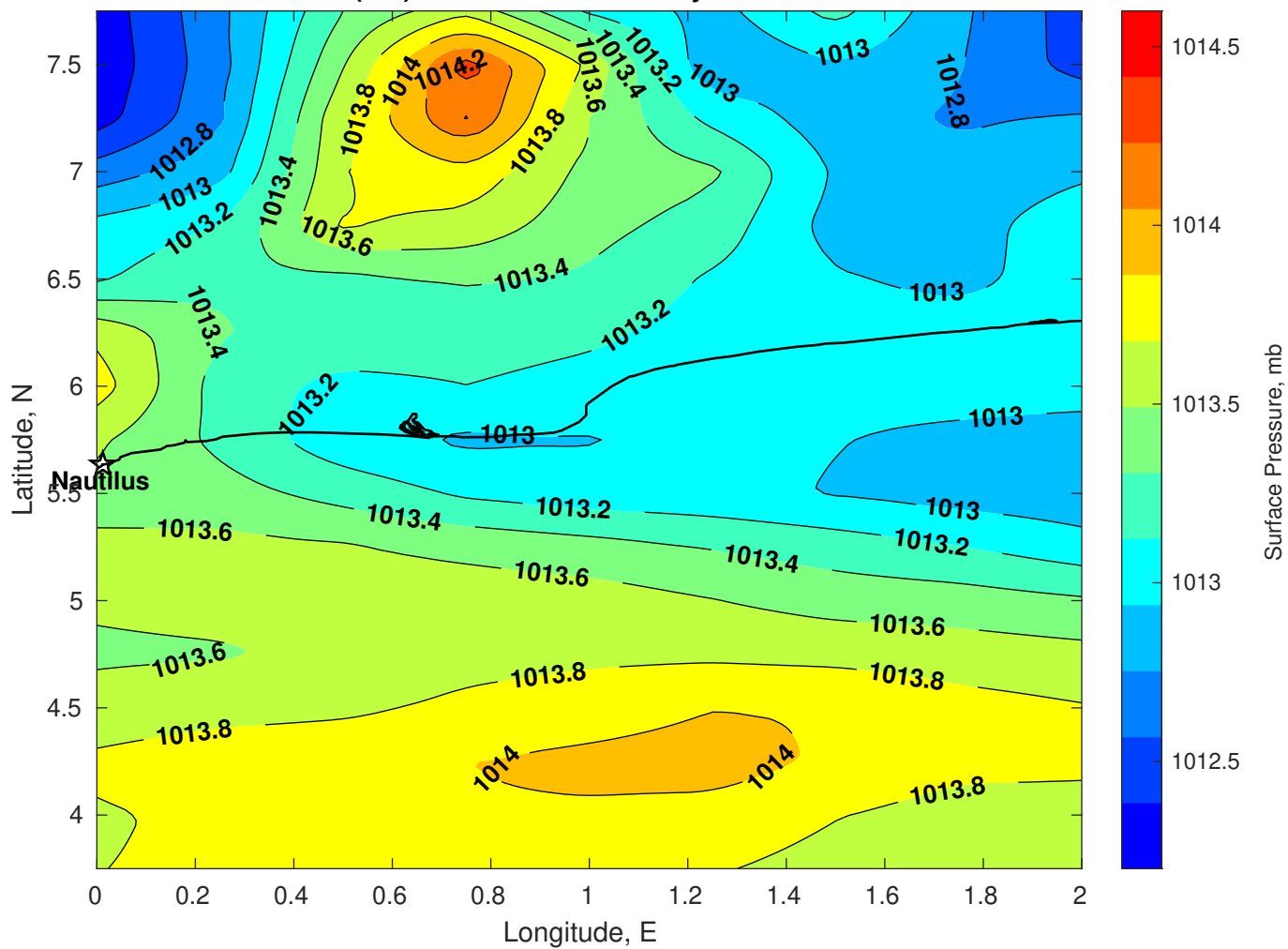
Surface Pressure (mb) for Nautilus at 27-May-2025 00:00:00
