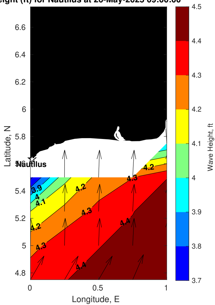
Wave Height (ft) for Nautilus at 26-May-2025 09:00:00
