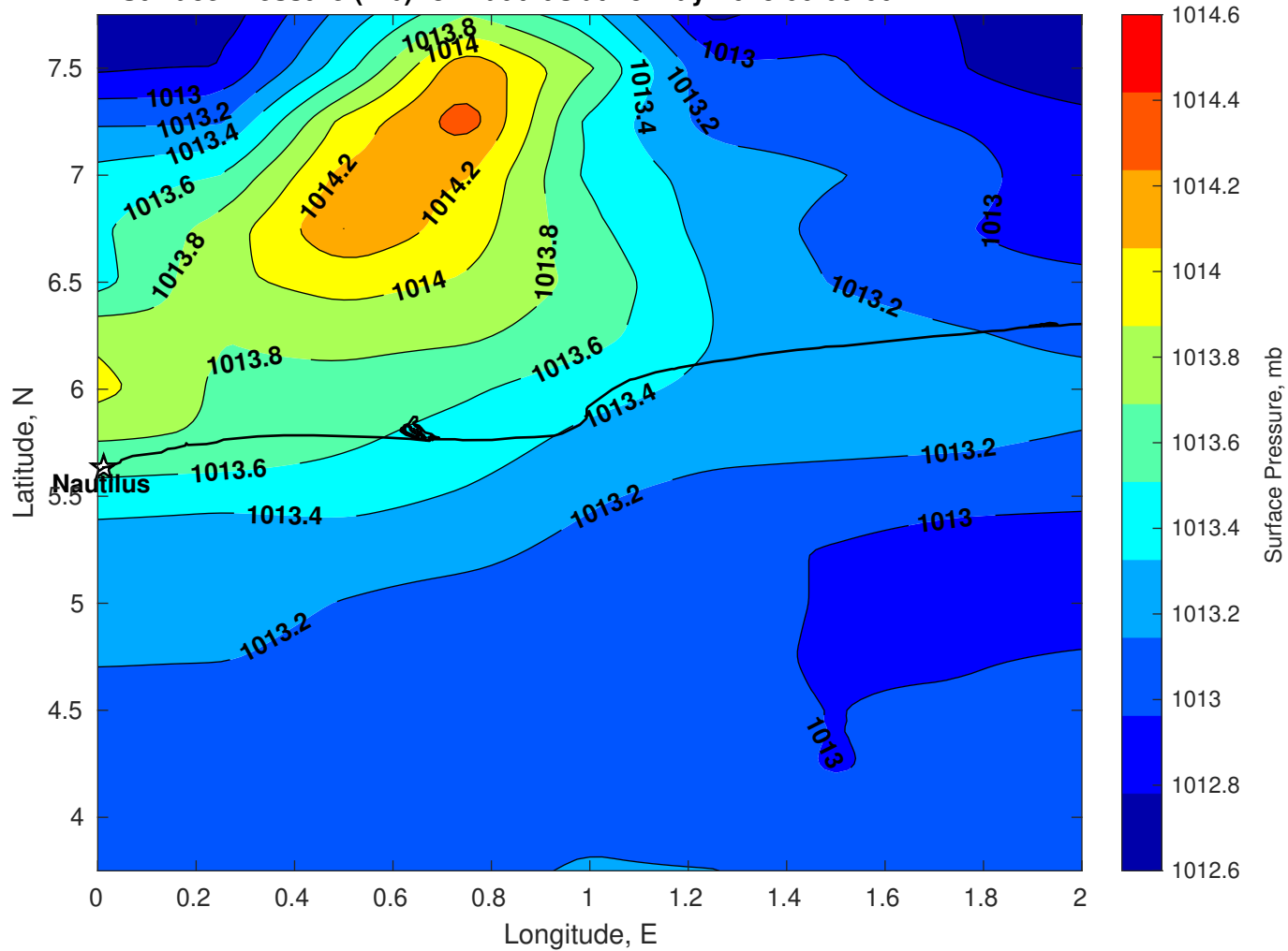
Surface Pressure (mb) for Nautilus at 28-May-2025 00:00:00
