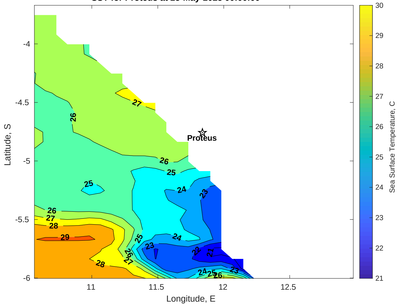
SST for Proteus at 25-May-2025 00:00:00
