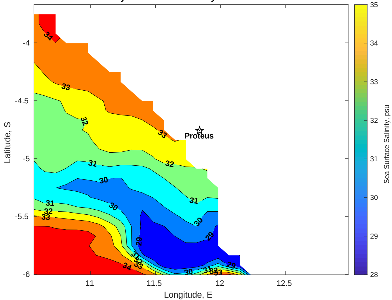
Surface Salinity for Proteus at 25-May-2025 00:00:00
