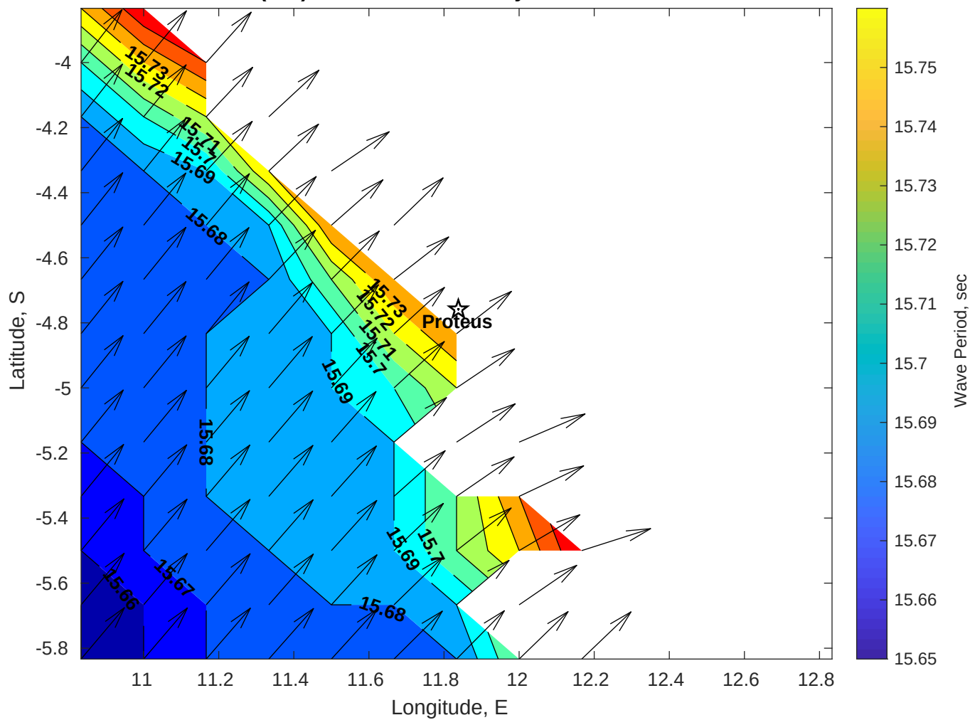
Wave Period (sec) for Proteus at 26-May-2025 09:00:00
