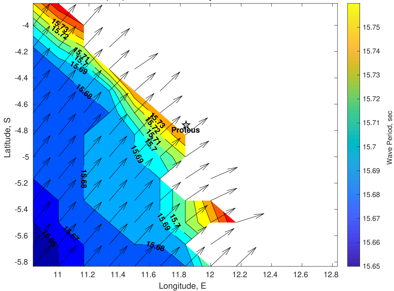
Wave Period (sec) for Proteus at 26-May-2025 09:00:00
