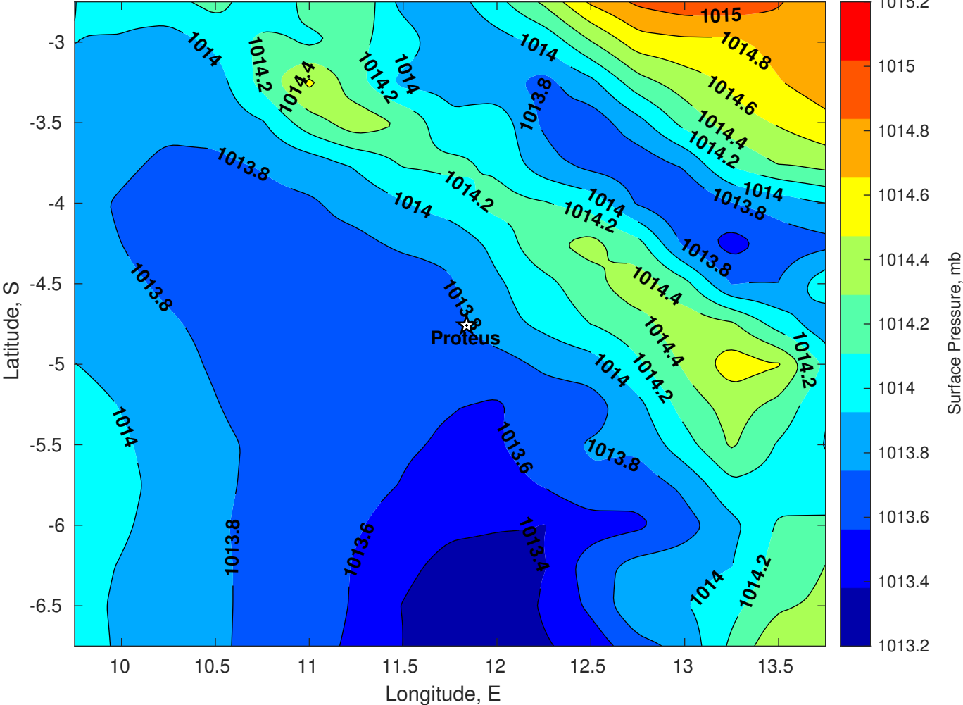
Surface Pressure (mb) for Proteus at 27-May-2025 00:00:00
