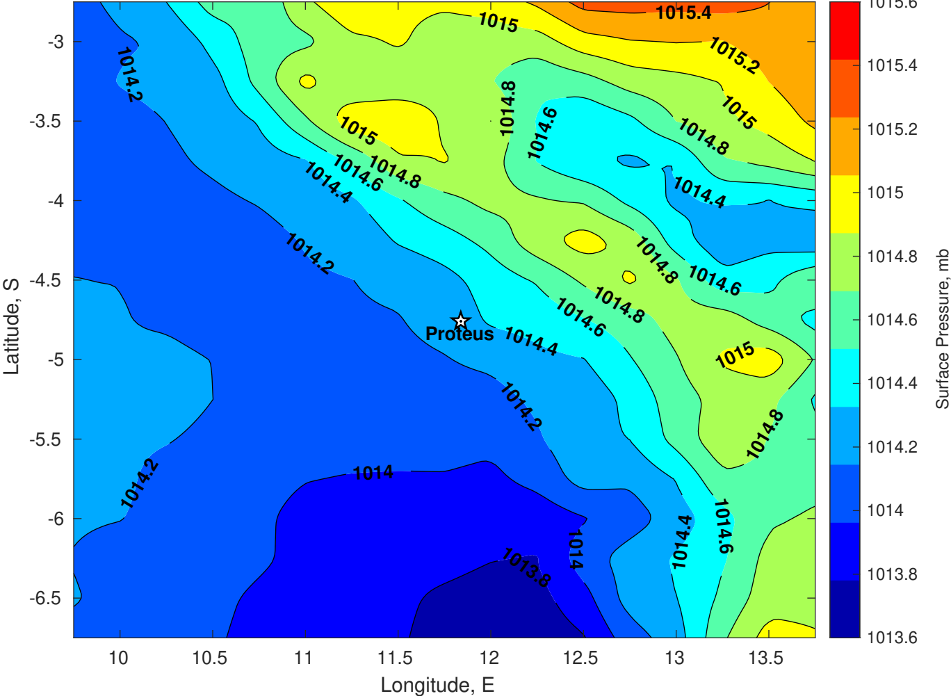
Surface Pressure (mb) for Proteus at 26-May-2025 00:00:00
