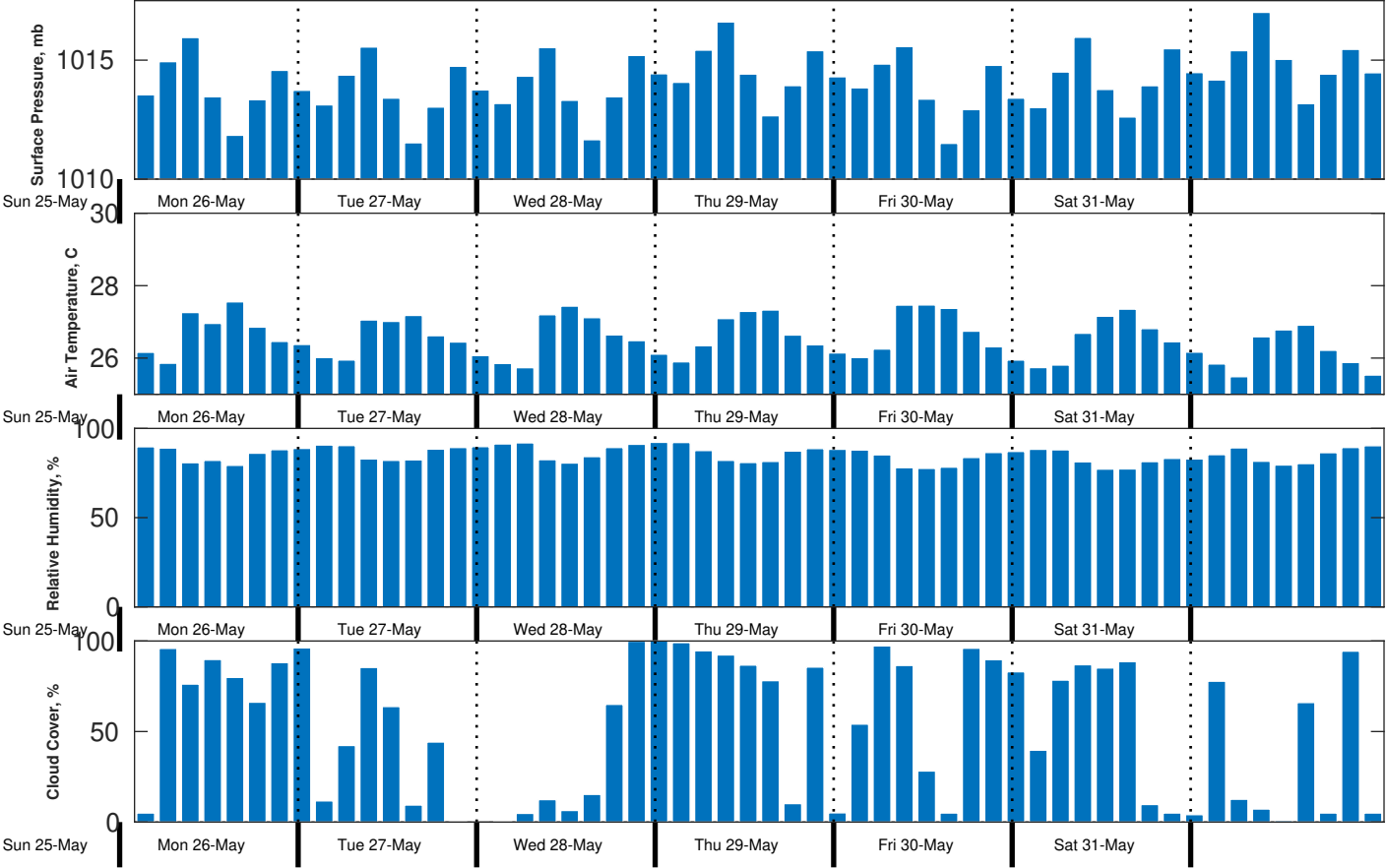
Met Forecast for Proteus from 26-May-2025 00:00:00 to 02-Jun-2025 00:00:00
