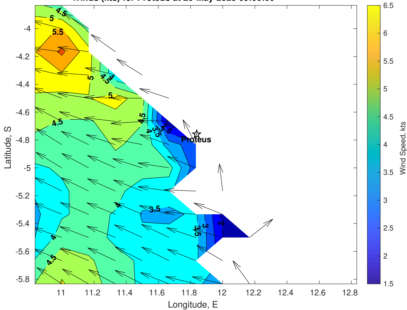
Winds (kts) for Proteus at 26-May-2025 09:00:00
