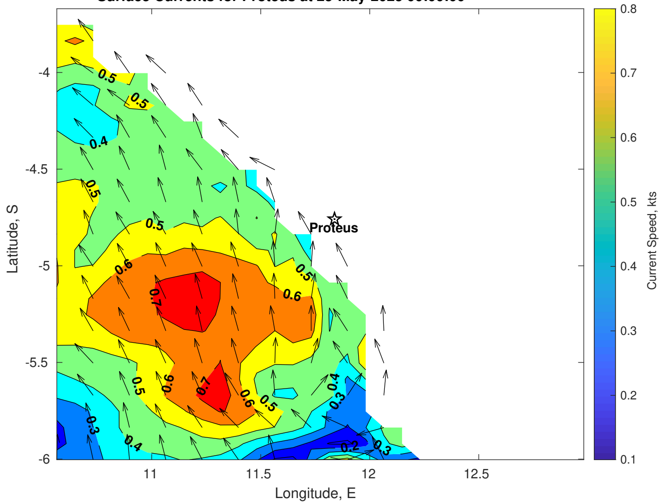
Surface Currents for Proteus at 25-May-2025 00:00:00
