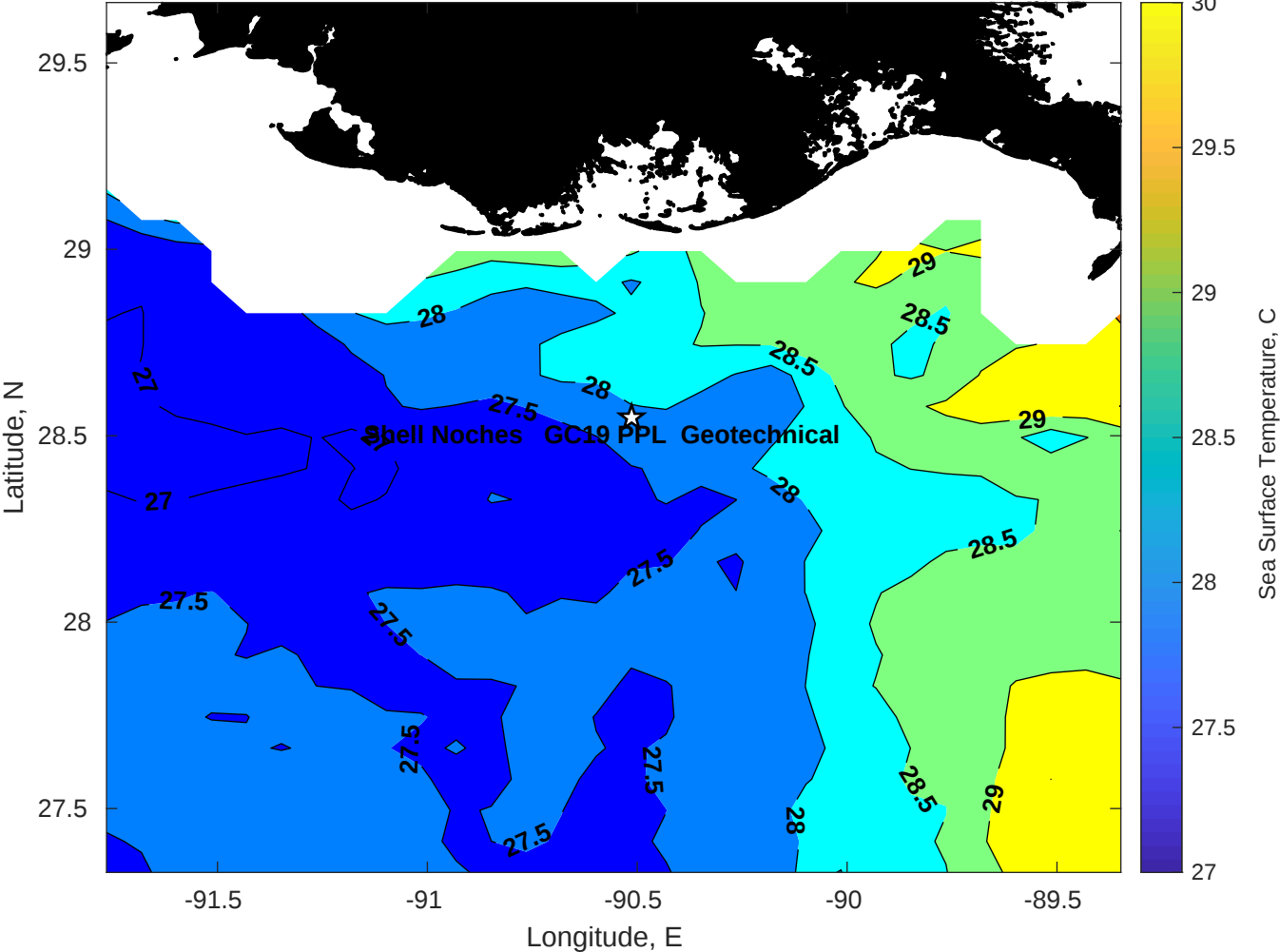
SST for Shell Noches GC19 PPL Geotechnical at 25-May-2025 00:00:00
