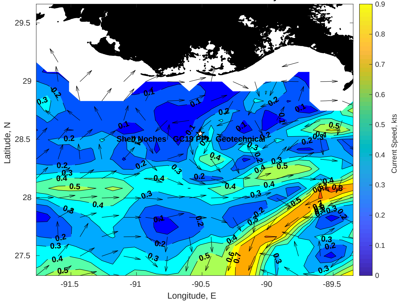
Surface Currents for Shell Noches GC19 PPL Geotechnical at 25-May-2025 00:00:00
