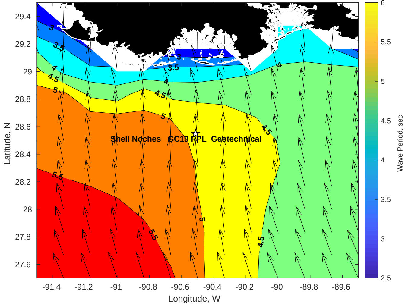
Wave Period (sec) for Shell Noches GC19 PPL Geotechnical at 26-May-2025 09:00:00
