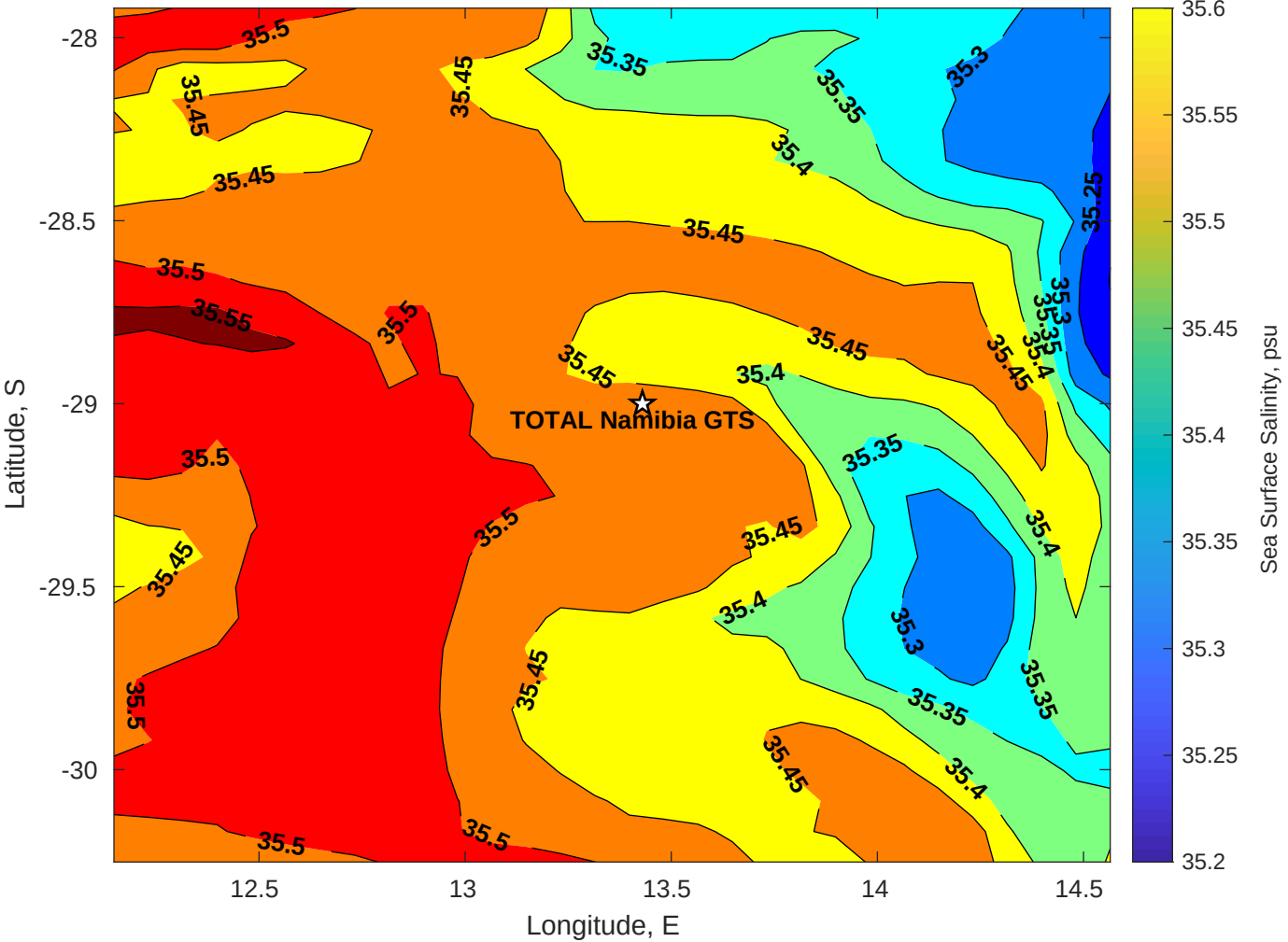
Surface Salinity for TOTAL Namibia GTS at 25-May-2025 00:00:00
