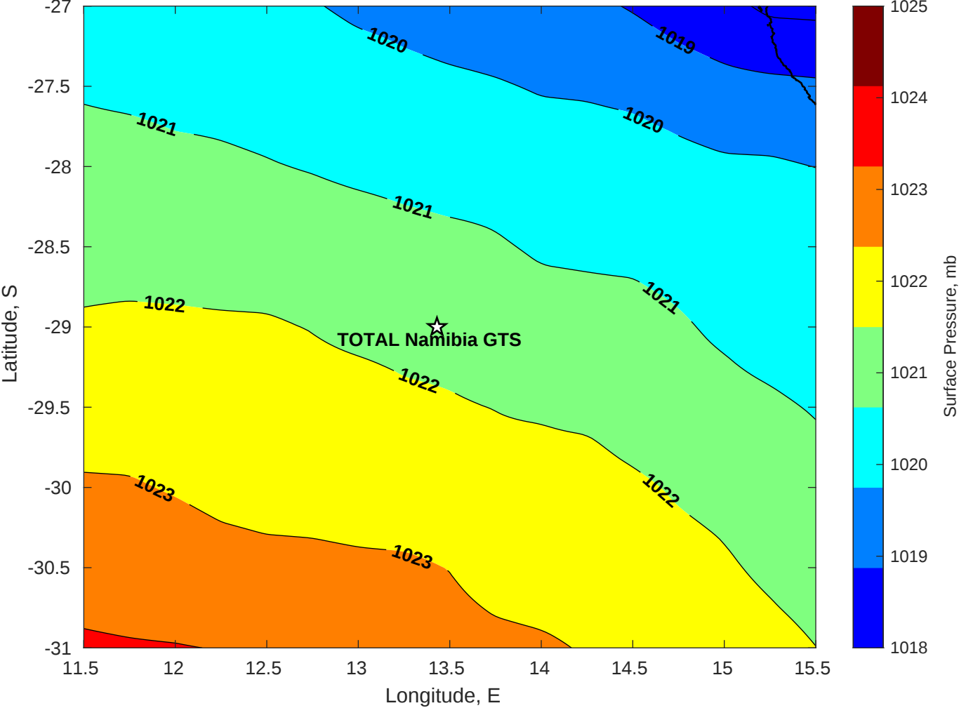
Surface Pressure (mb) for TOTAL Namibia GTS at 27-May-2025 00:00:00
