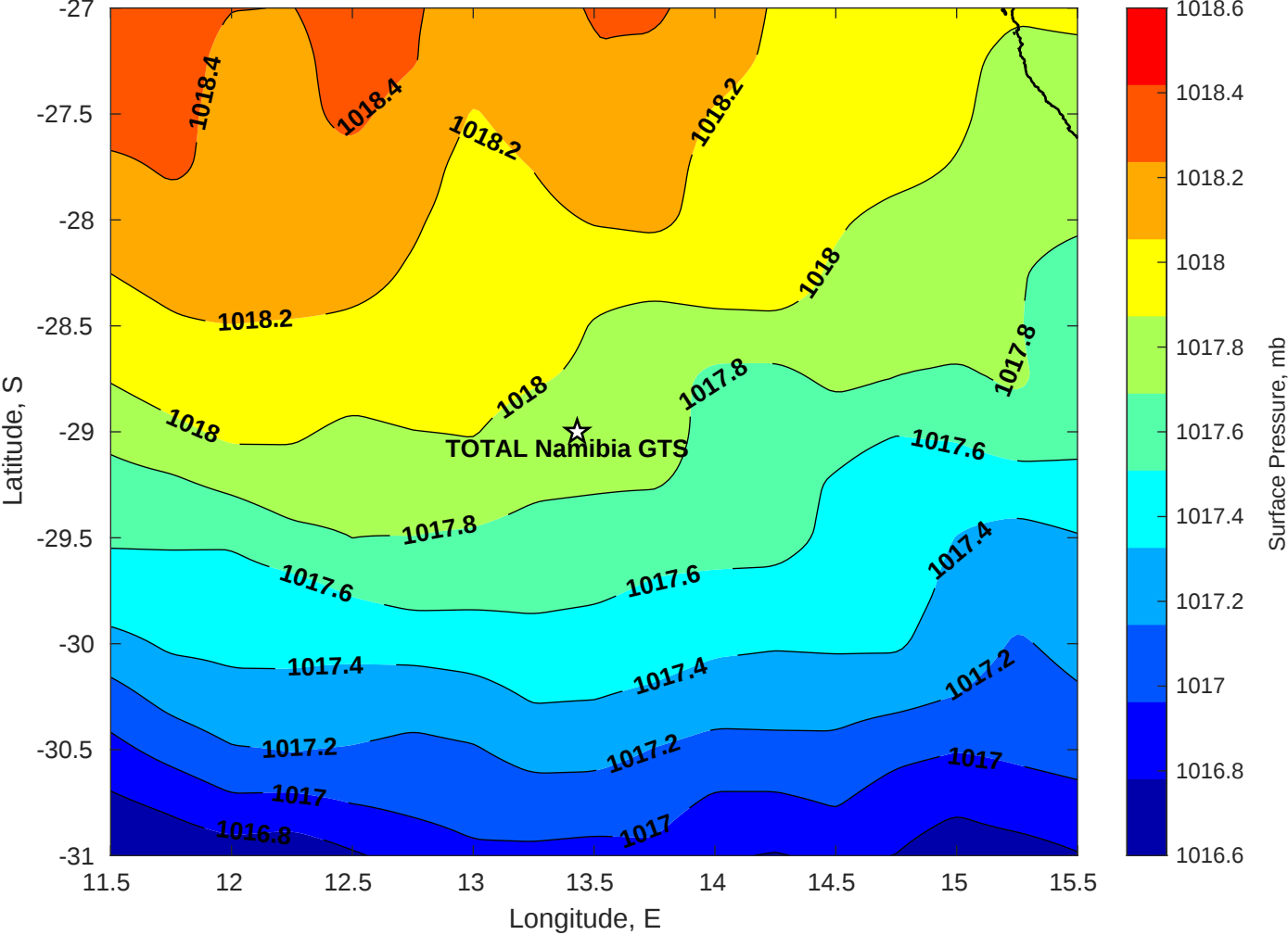
Surface Pressure (mb) for TOTAL Namibia GTS at 28-May-2025 00:00:00
