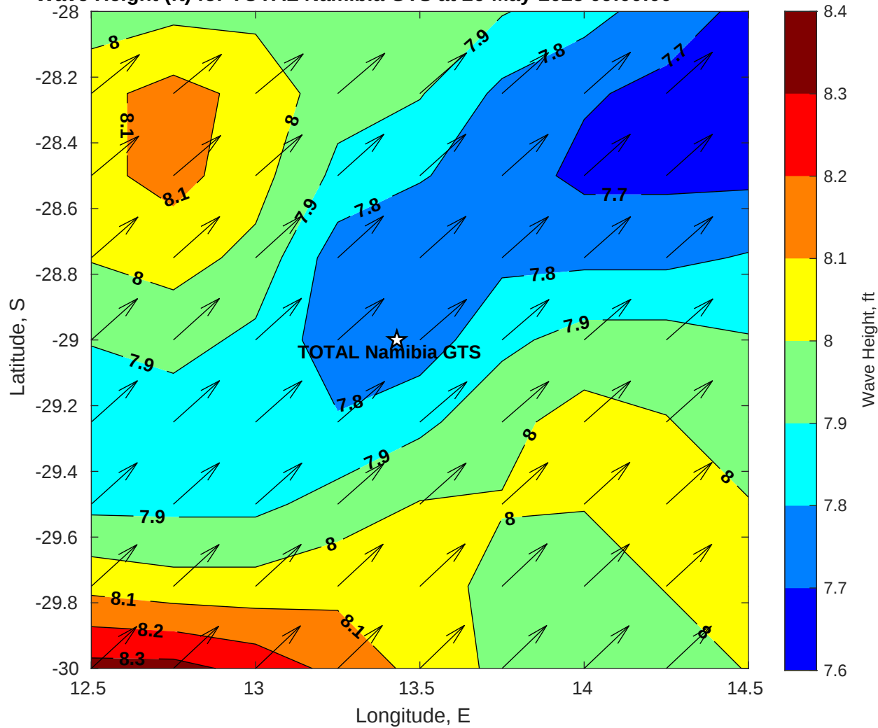
Wave Height (ft) for TOTAL Namibia GTS at 26-May-2025 09:00:00
