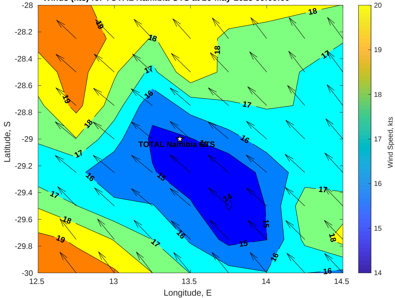
Winds (kts) for TOTAL Namibia GTS at 26-May-2025 09:00:00
