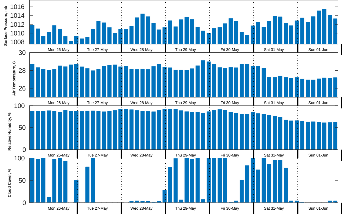
Met Forecast for Tampnet P2378 South Texas Cable Route Geophysical from 26-May-2025 00:00:00 to 02-Jun-2025 00:00:00
