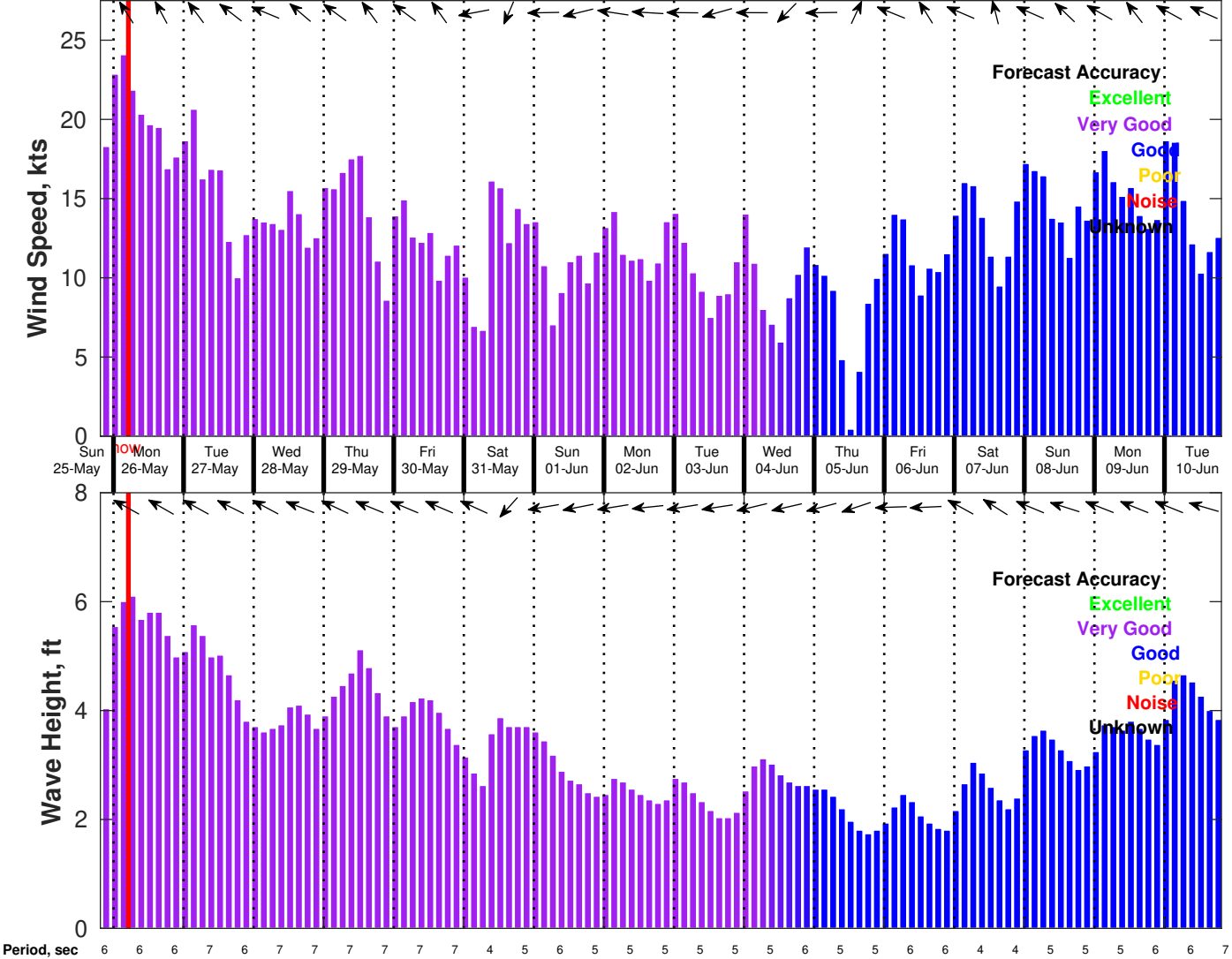
Wind & Wave Forecast for Tampnet P2378 South Texas Cable Route Geophysical from 25-May-2025 20:00:00 to 10-Jun-2025 20:00:00
