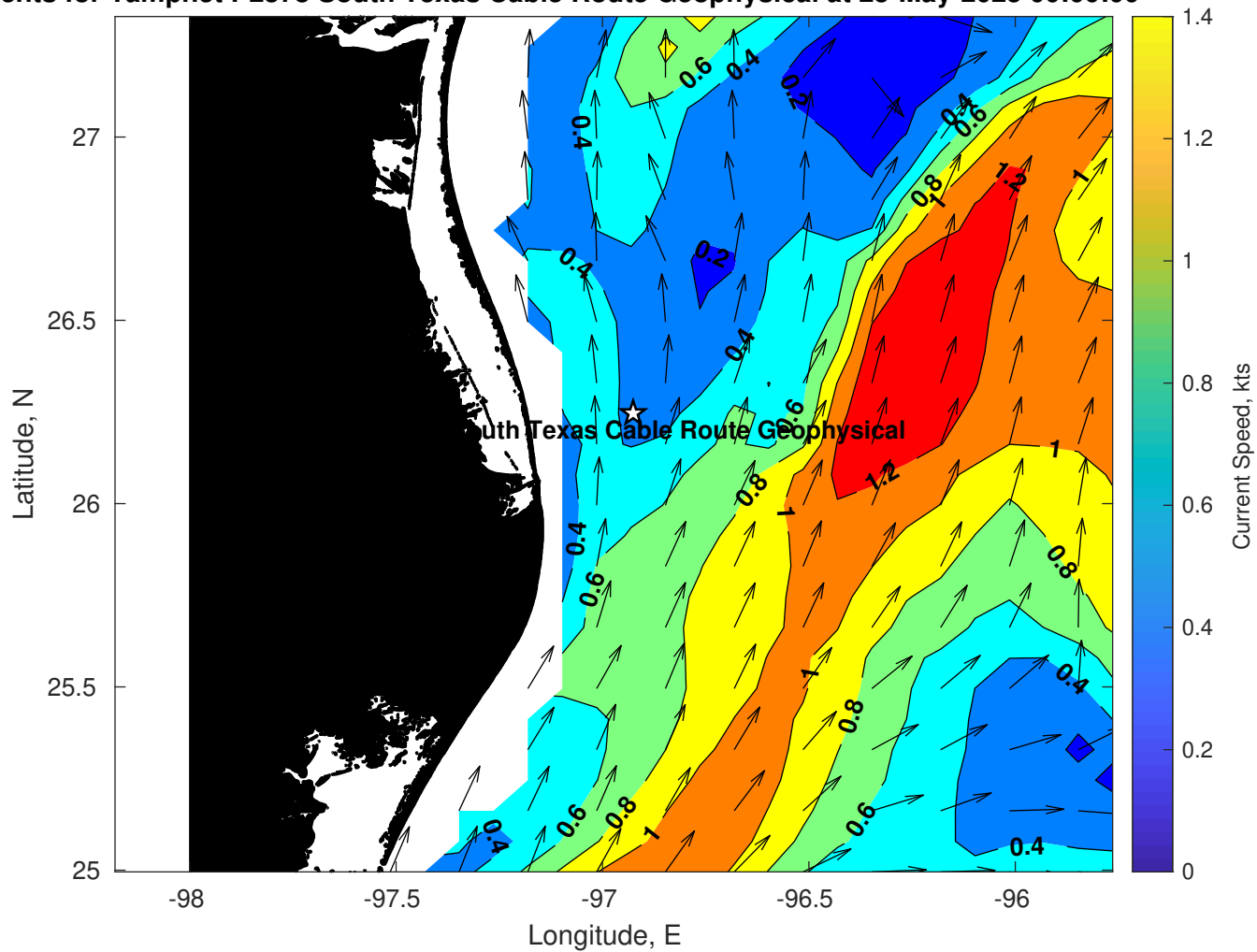
Surface Currents for Tampnet P2378 South Texas Cable Route Geophysical at 25-May-2025 00:00:00
