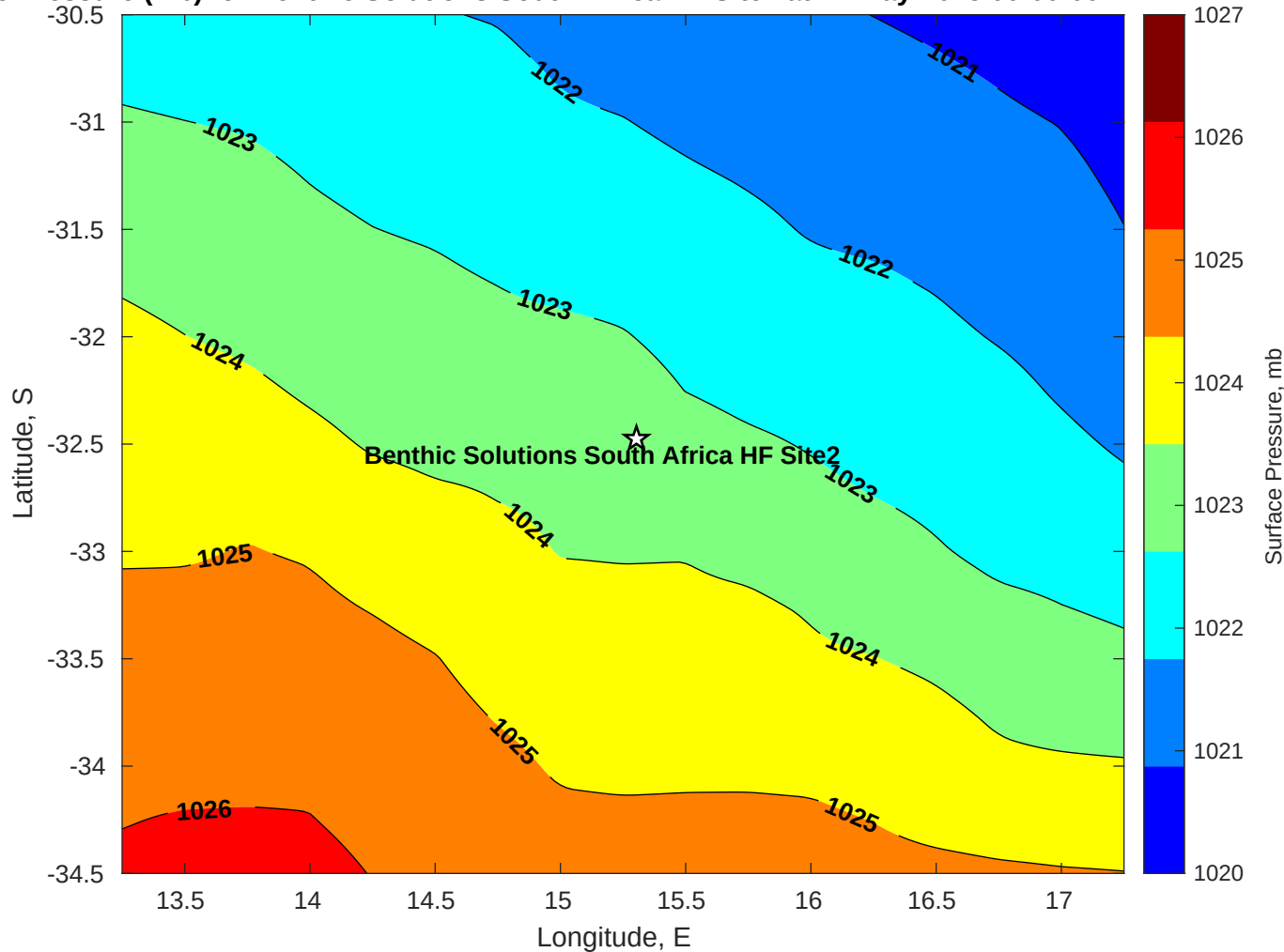
Surface Pressure (mb) for Benthic Solutions South Africa HF Site2 at 27-May-2025 00:00:00
