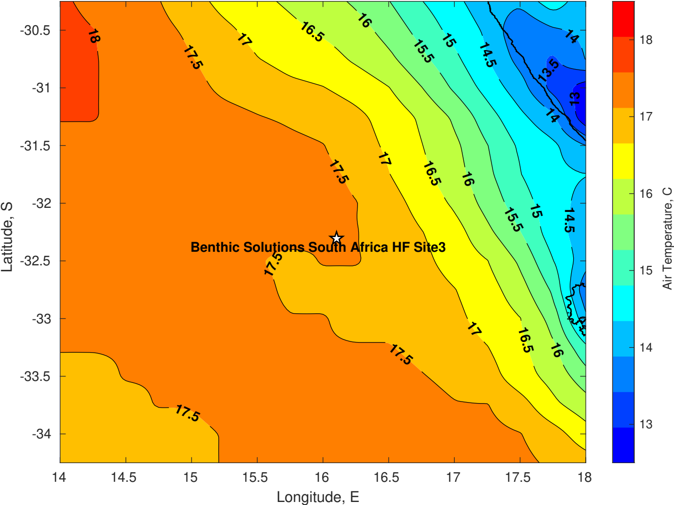
Air Temperature (C) for Benthic Solutions South Africa HF Site3 at 27-May-2025
