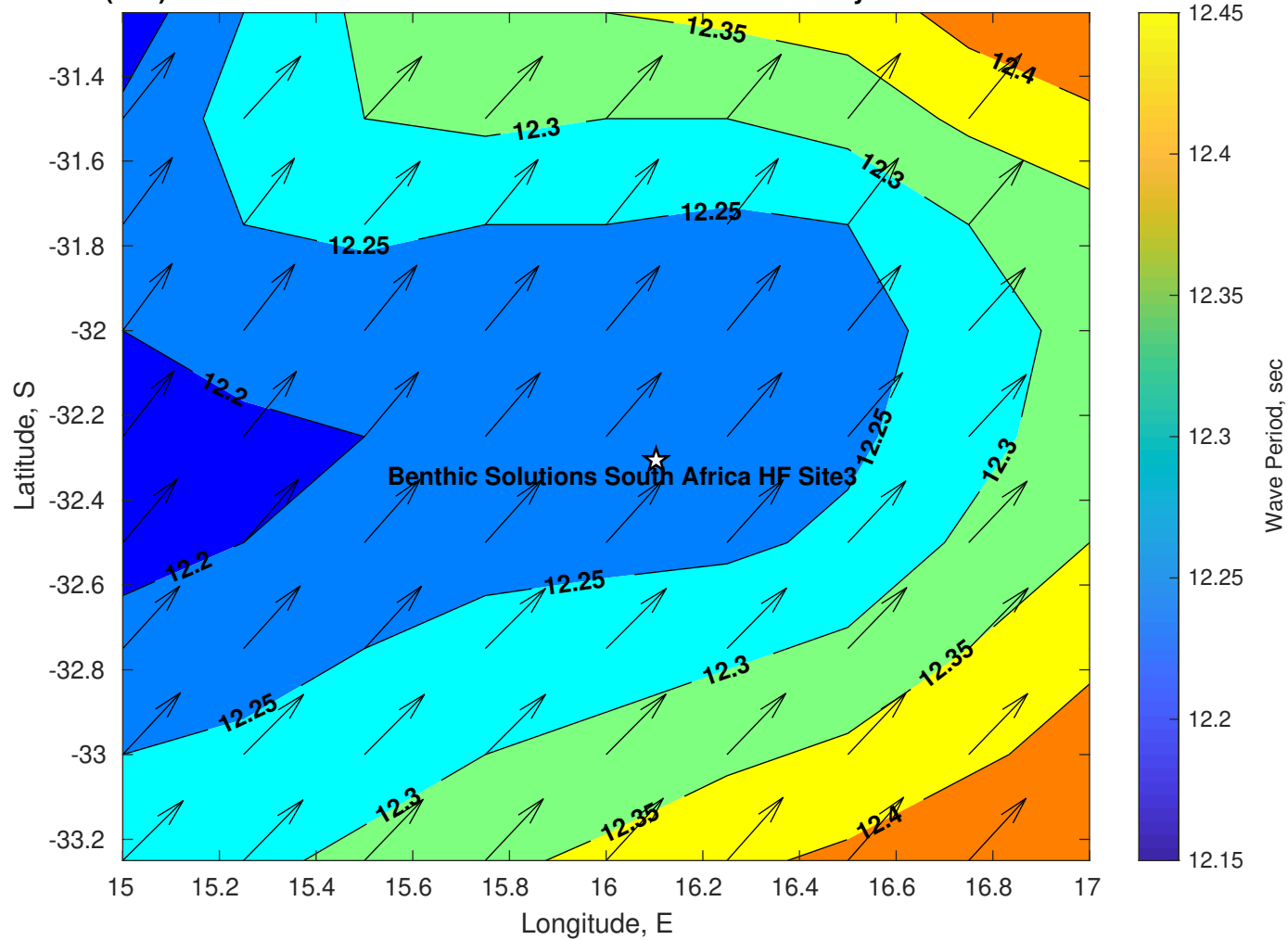
Wave Period (sec) for Benthic Solutions South Africa HF Site3 at 27-May-2025 09:00:00
