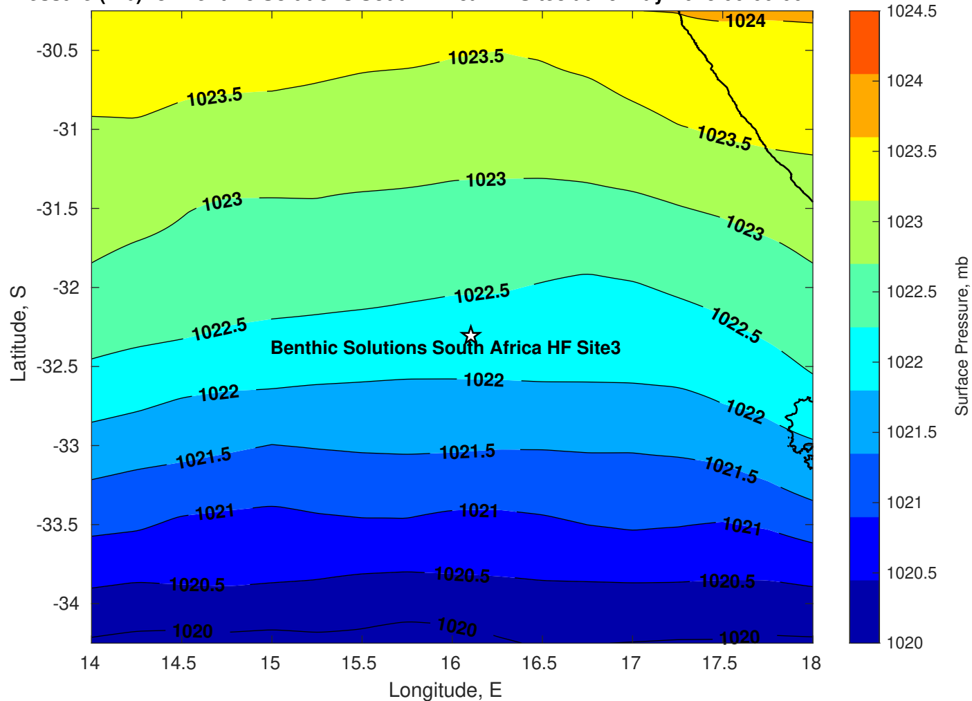
Surface Pressure (mb) for Benthic Solutions South Africa HF Site3 at 29-May-2025 00:00:00
