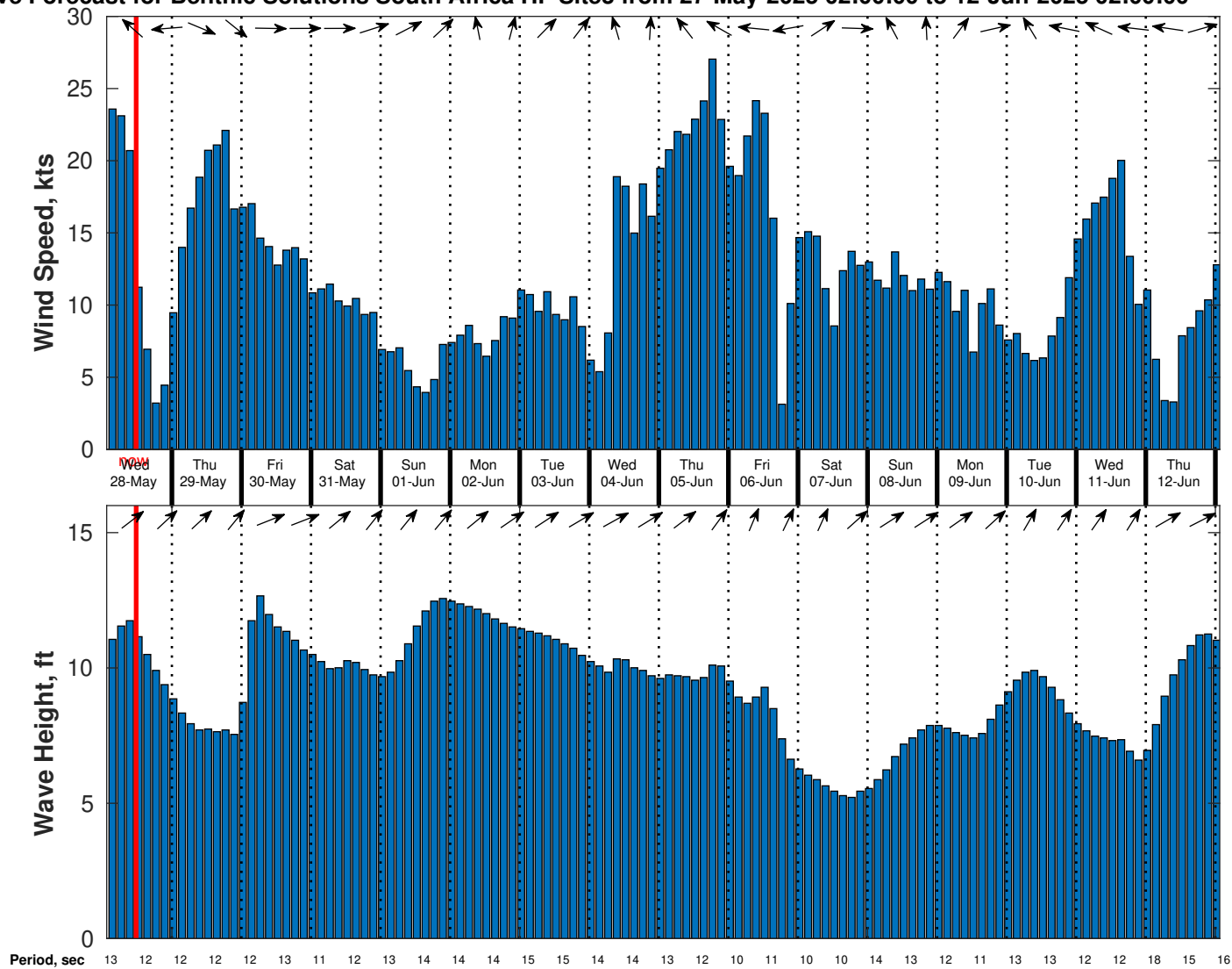
Wind & Wave Forecast for Benthic Solutions South Africa HF Site3 from 27-May-2025 02:00:00 to 12-Jun-2025 02:00:00
