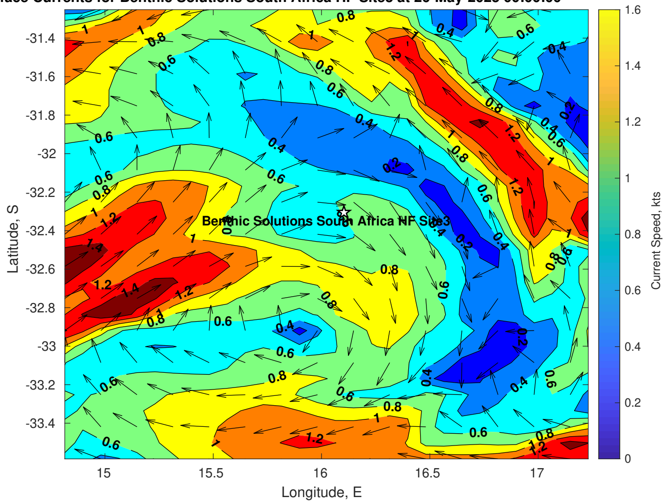
Surface Currents for Benthic Solutions South Africa HF Site3 at 26-May-2025 00:00:00
