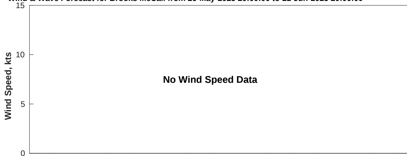
Wind & Wave Forecast for Brooks McCall from 26-May-2025 20:00:00 to 11-Jun-2025 20:00:00
