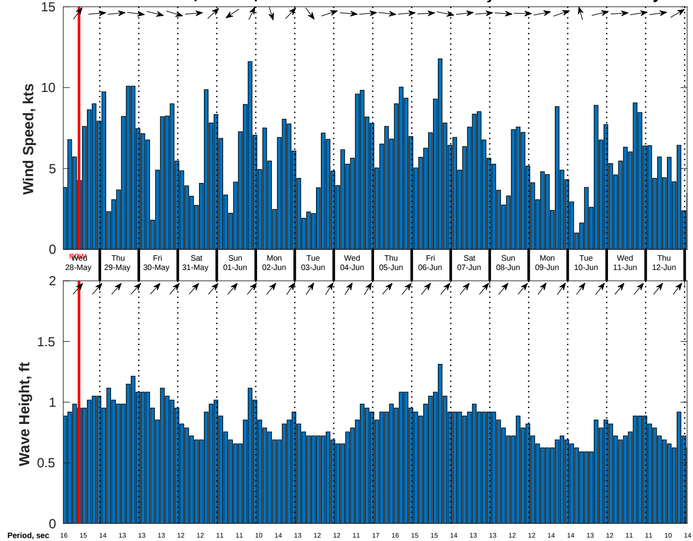
Wind & Wave Forecast for CSA (ONHYM) PPL EBS - Guinea from 27-May-2025 01:00:00 to 12-Jun-2025 01:00:00
