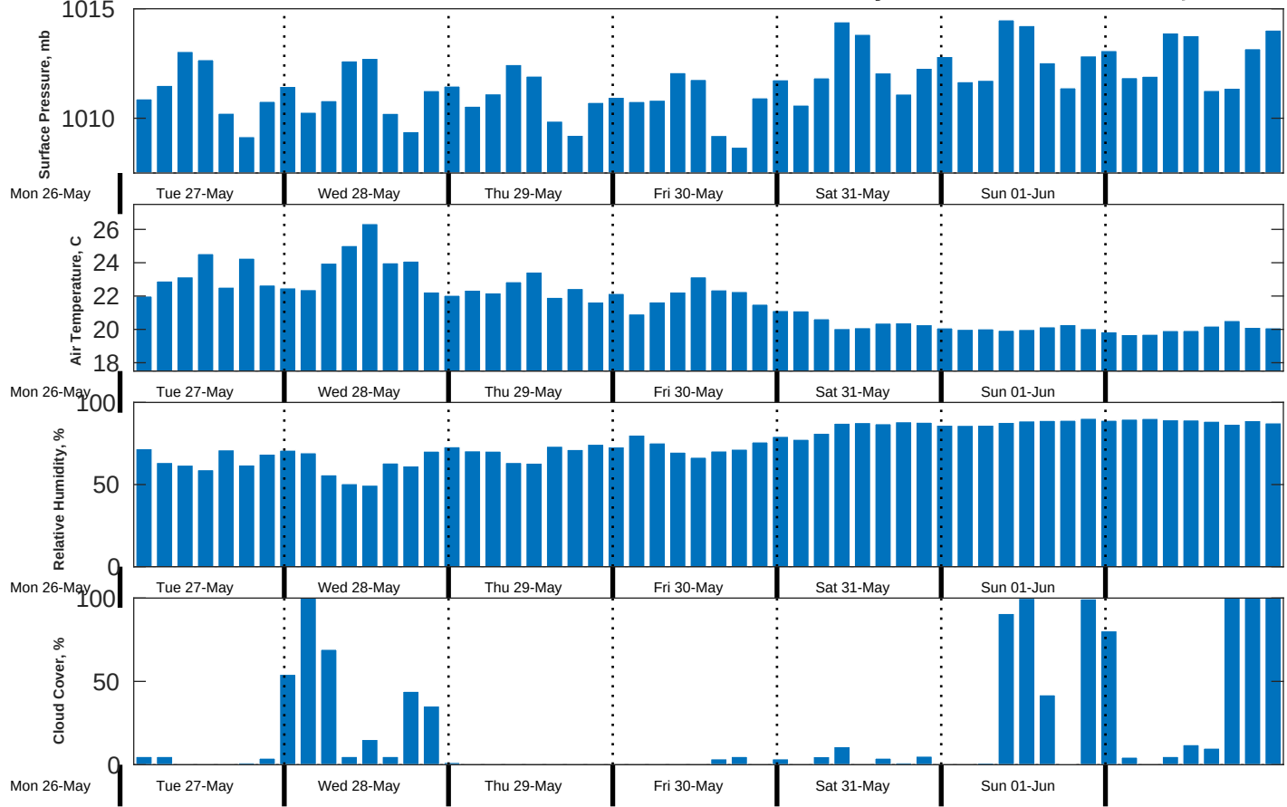
Met Forecast for CSA (ONHYM) PPL EBS - Mauritania from 27-May-2025 00:00:00 to 03-Jun-2025 00:00:00
