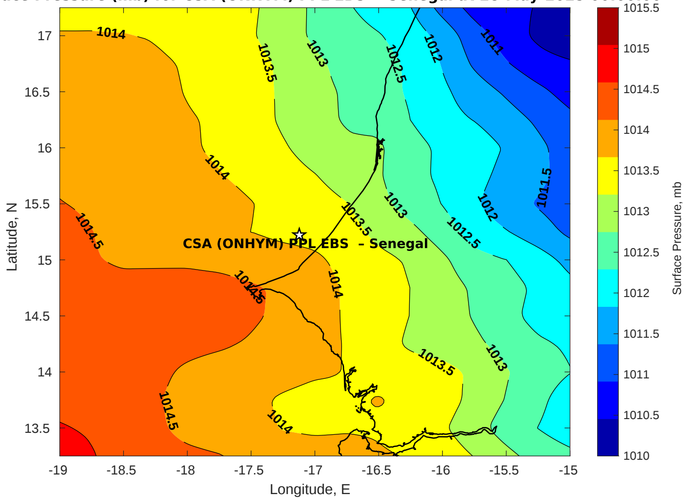
Surface Pressure (mb) for CSA (ONHYM) PPL EBS - Senegal at 28-May-2025 00:00:00
