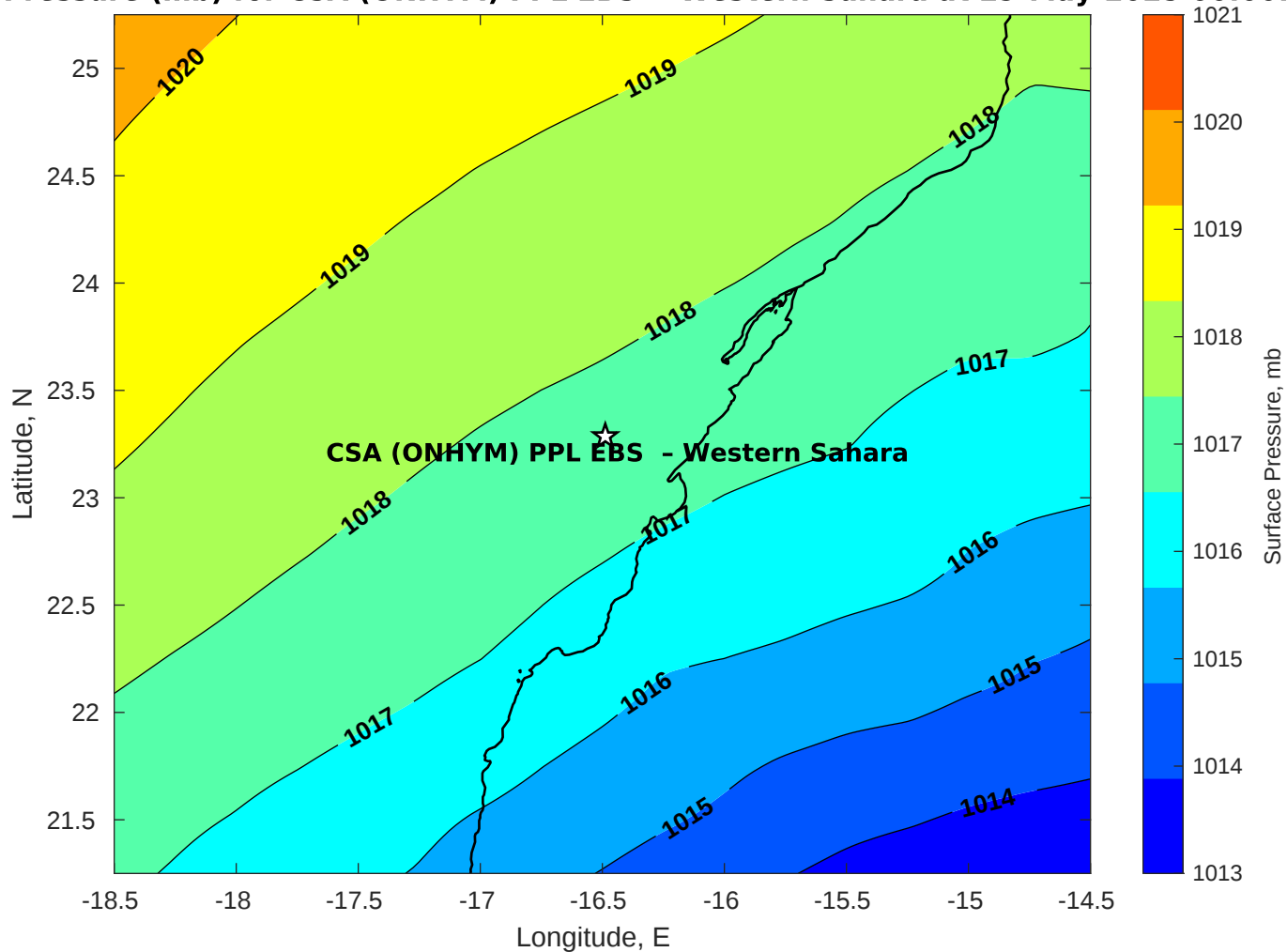
Surface Pressure (mb) for CSA (ONHYM) PPL EBS - Western Sahara at 29-May-2025 00:00:00
