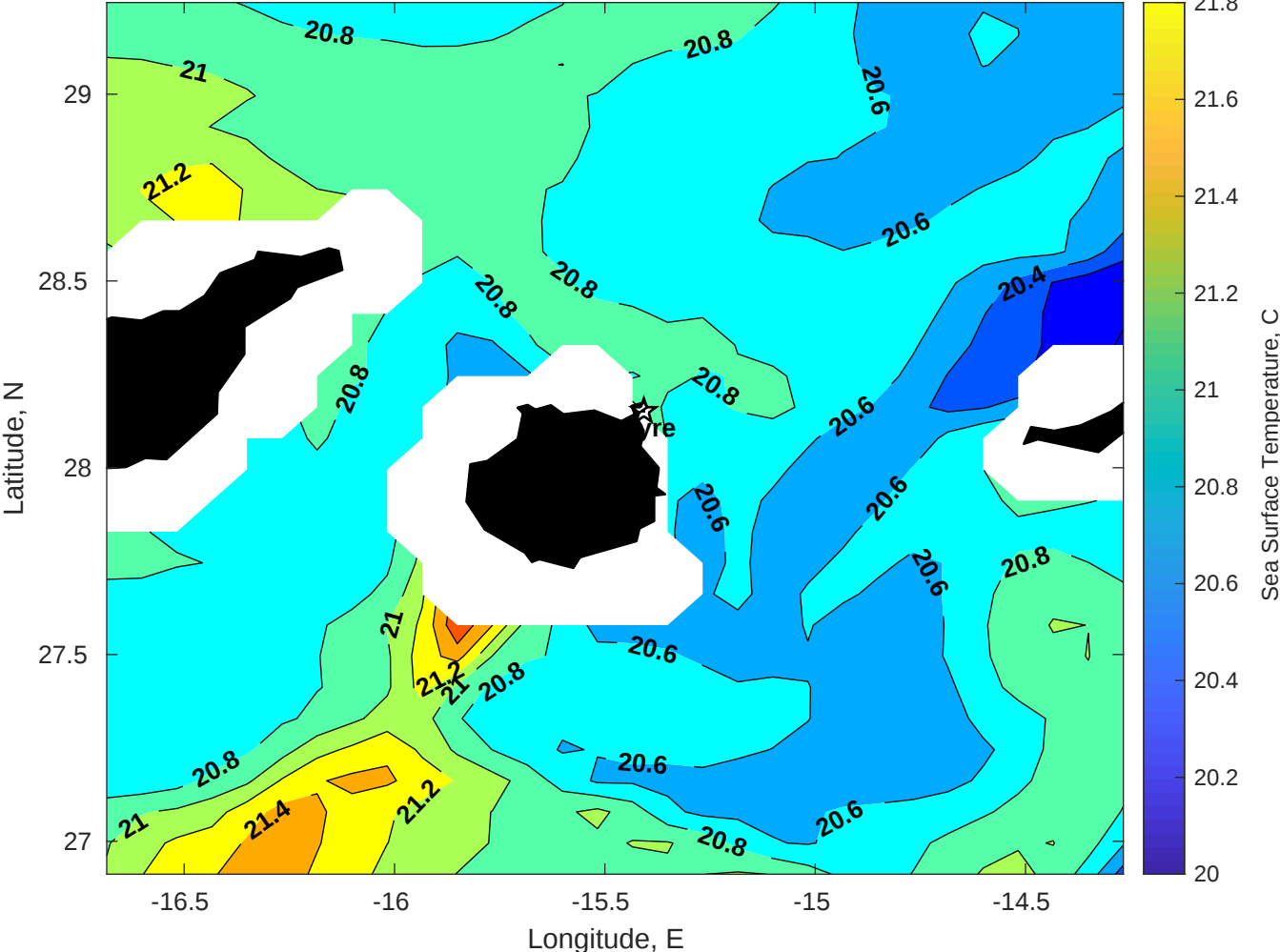
SST for Gyre at 26-May-2025 00:00:00
