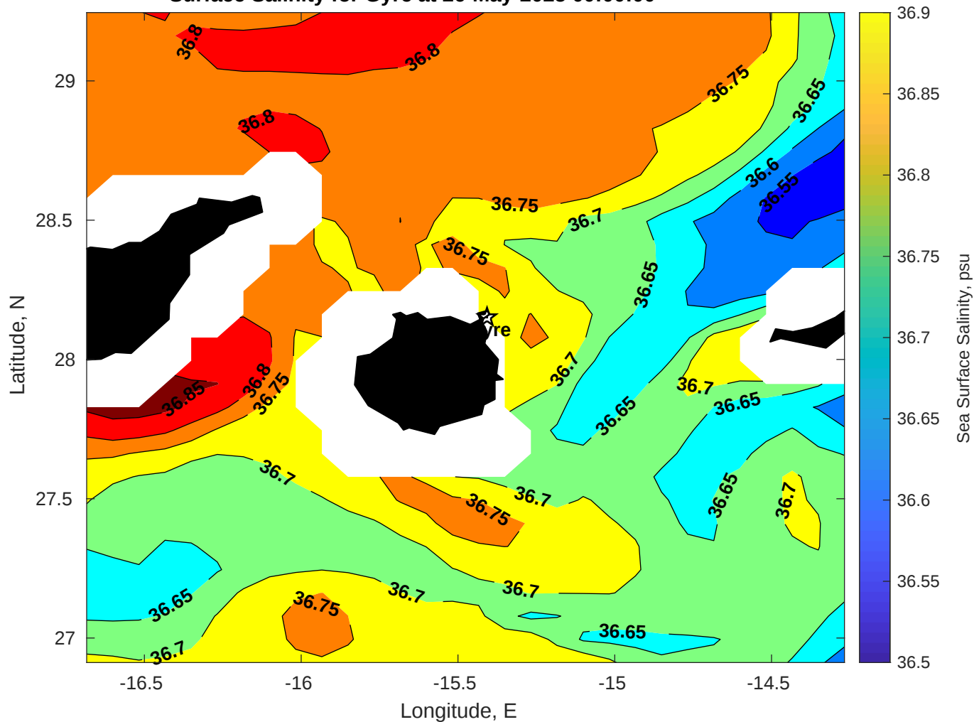
Surface Salinity for Gyre at 26-May-2025 00:00:00
