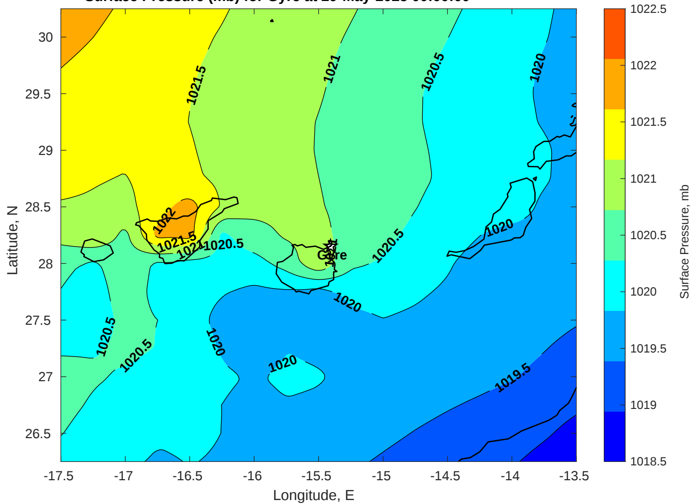
Surface Pressure (mb) for Gyre at 29-May-2025 00:00:00
