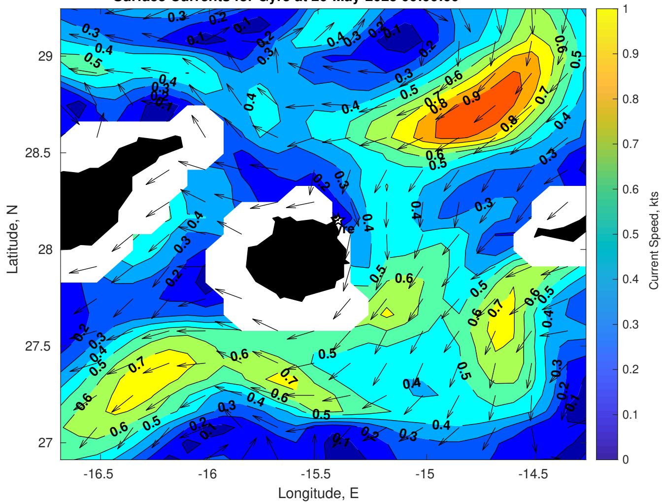
Surface Currents for Gyre at 26-May-2025 00:00:00
