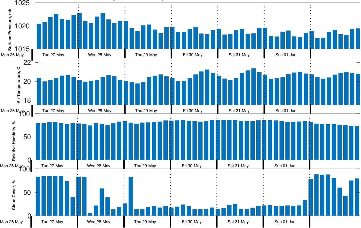
Met Forecast for Gyre from 26-May-2025 23:00:00 to 02-Jun-2025 23:00:00
