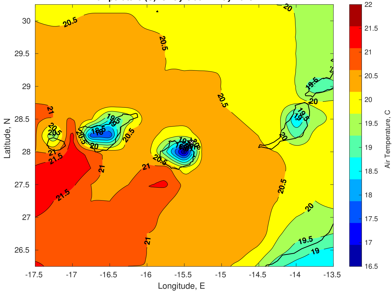
Air Temperature (C) for Gyre at 27-May-2025
