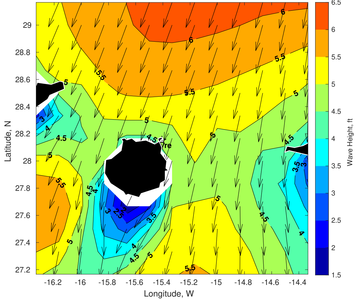
Wave Height (ft) for Gyre at 27-May-2025 09:00:00
