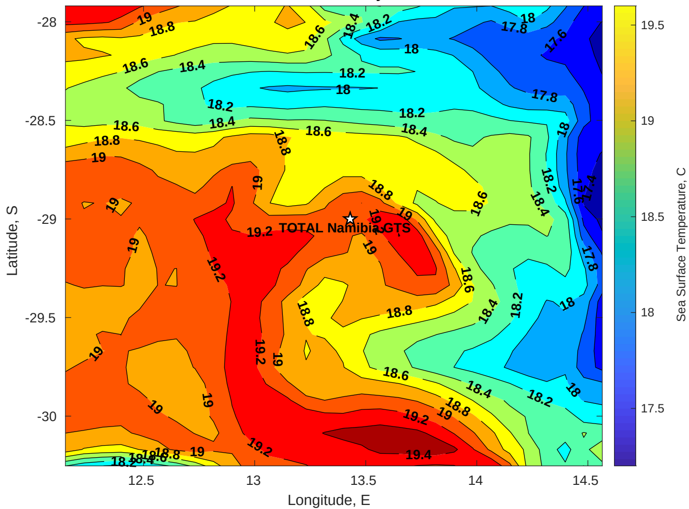
SST for TOTAL Namibia GTS at 26-May-2025 00:00:00
