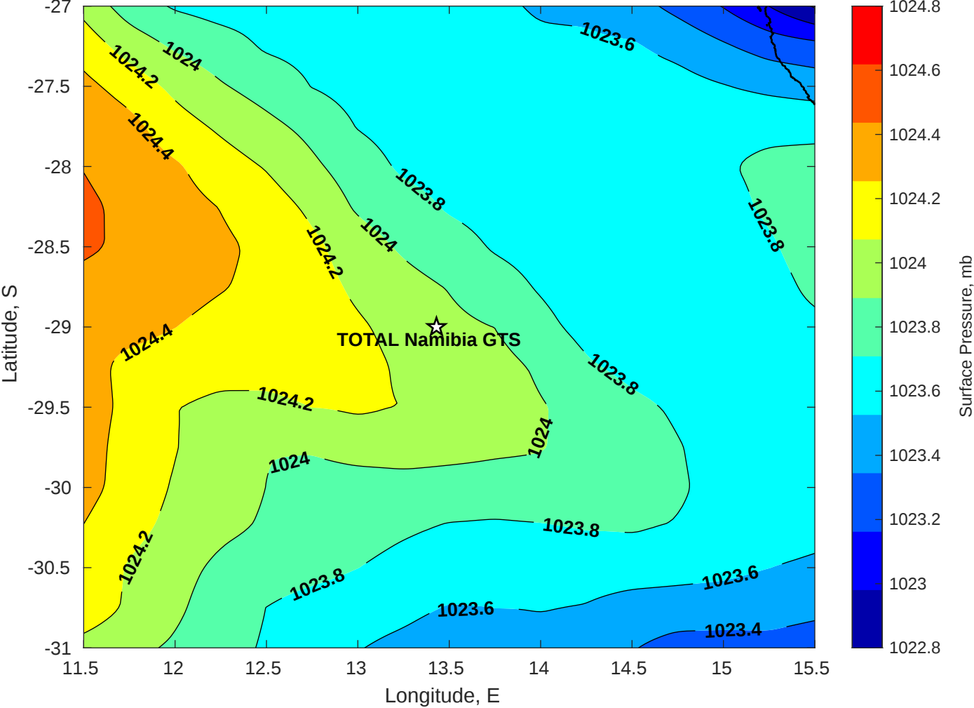
Surface Pressure (mb) for TOTAL Namibia GTS at 29-May-2025 00:00:00
