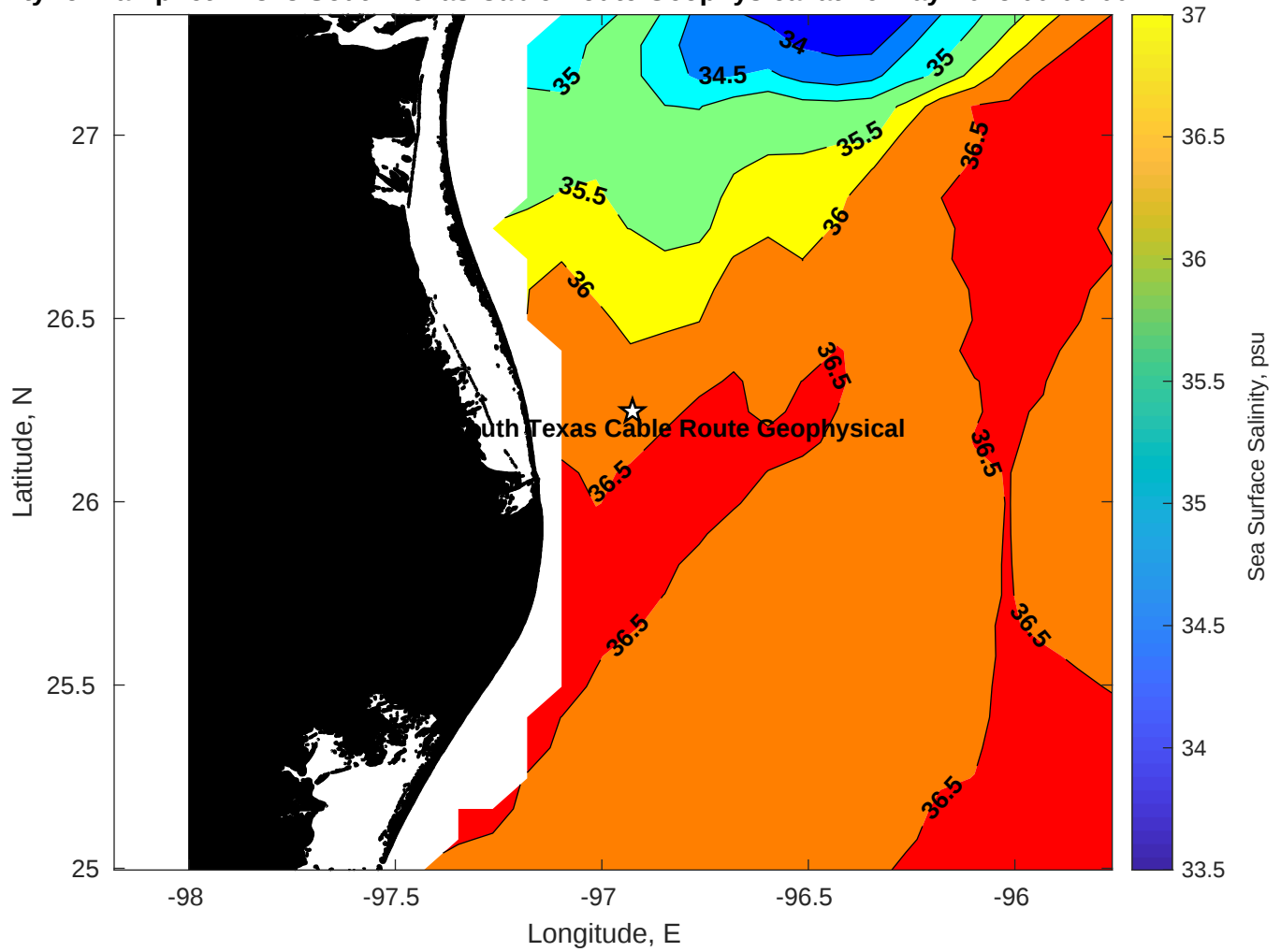
Surface Salinity for Tampnet P2378 South Texas Cable Route Geophysical at 26-May-2025 00:00:00
