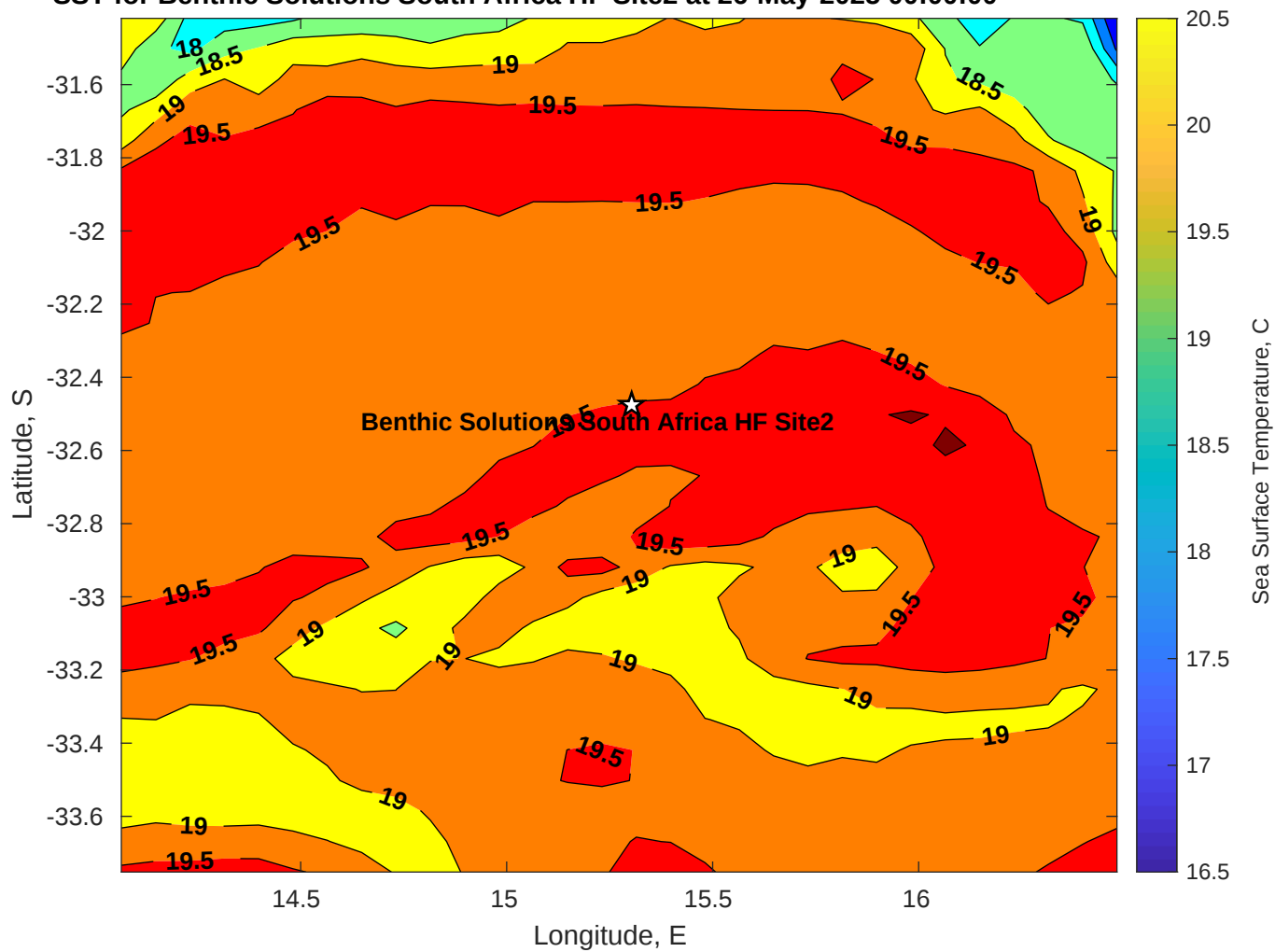
SST for Benthic Solutions South Africa HF Site2 at 26-May-2025 00:00:00
