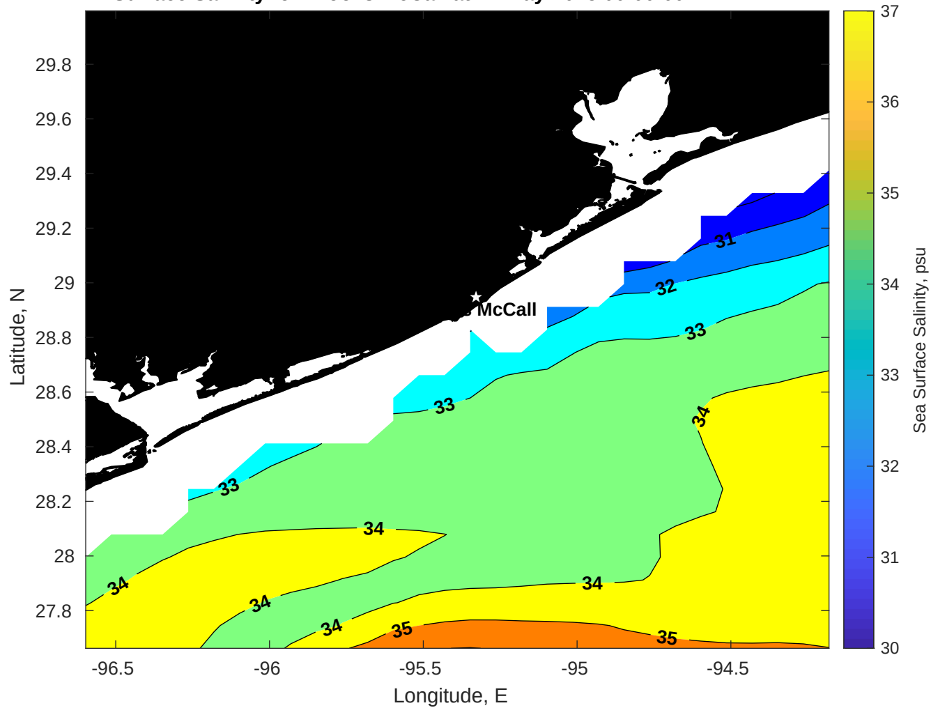
Surface Salinity for Brooks McCall at 27-May-2025 00:00:00
