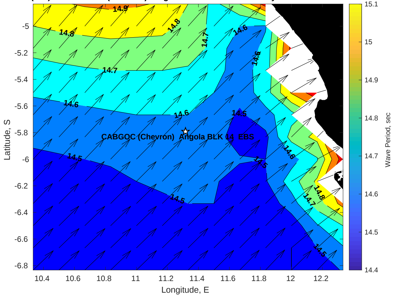
Wave Period (sec) for CABGOC (Chevron) Angola BLK 14 EBS at 27-May-2025 09:00:00
