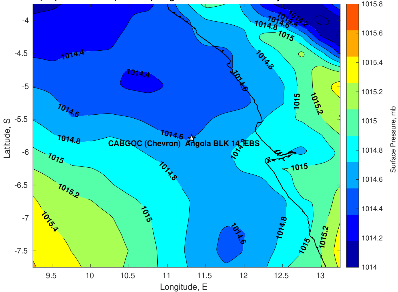
Surface Pressure (mb) for CABGOC (Chevron) Angola BLK 14 EBS at 29-May-2025 00:00:00
