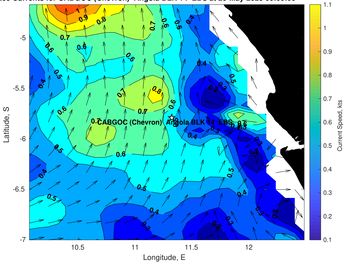
Surface Currents for CABGOC (Chevron) Angola BLK 14 EBS at 26-May-2025 00:00:00
