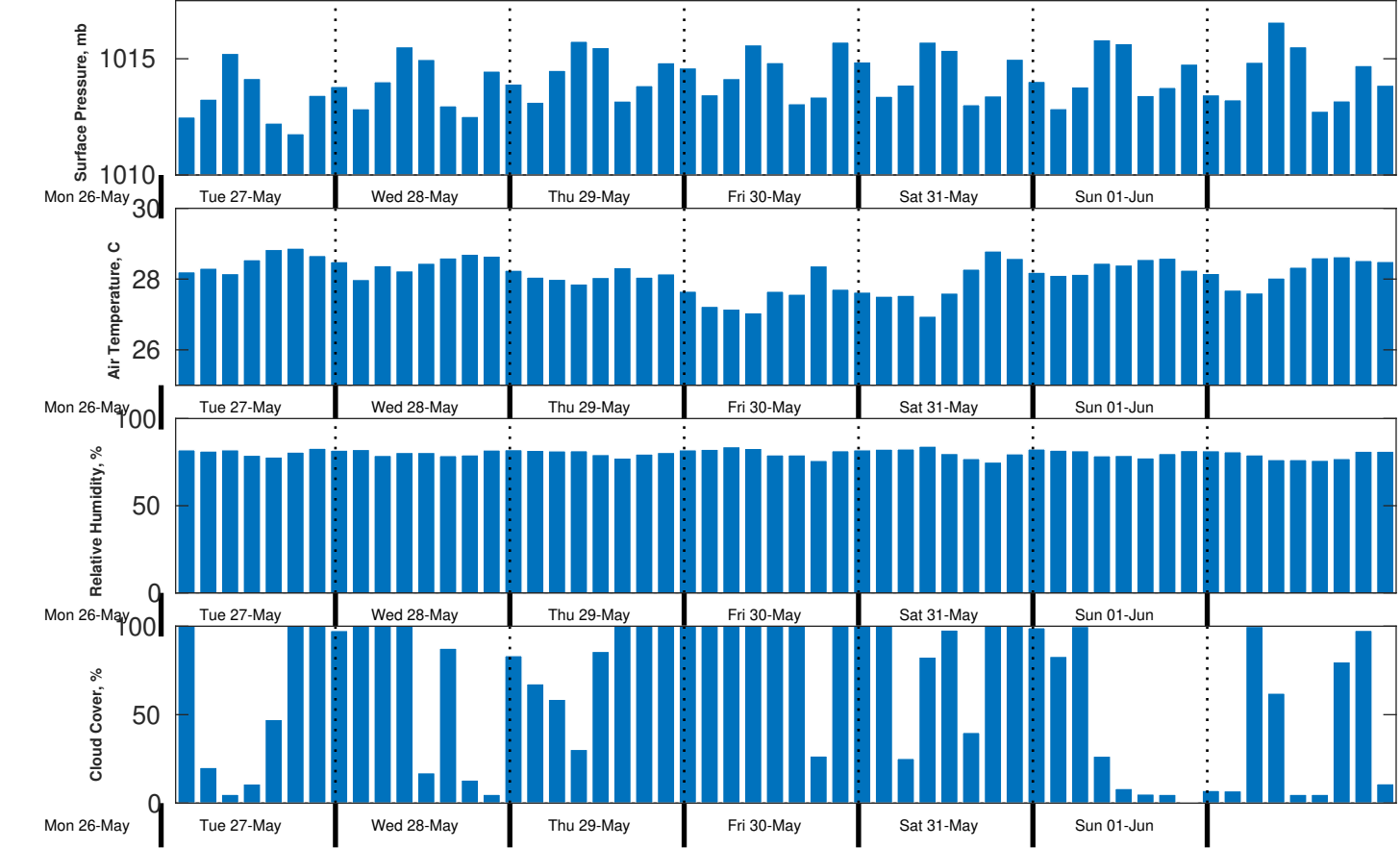
Met Forecast for CSA (ONHYM) PPL EBS - Cote d'Ivoire from 27-May-2025 00:00:00 to 03-Jun-2025 00:00:00
