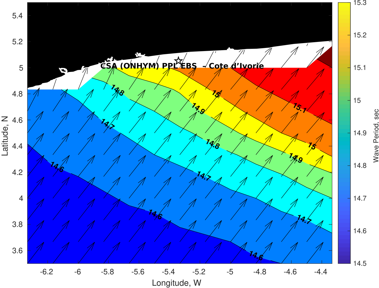
Wave Period (sec) for CSA (ONHYM) PPL EBS - Cote d'Ivoire at 27-May-2025 09:00:00
