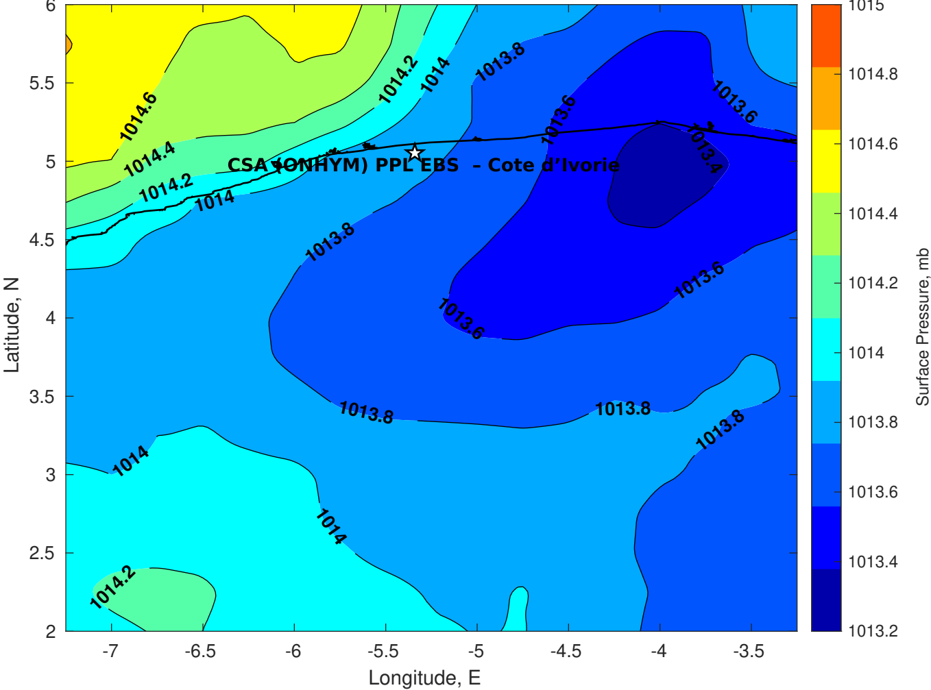
Surface Pressure (mb) for CSA (ONHYM) PPL EBS - Cote d'Ivoire at 28-May-2025 00:00:00
