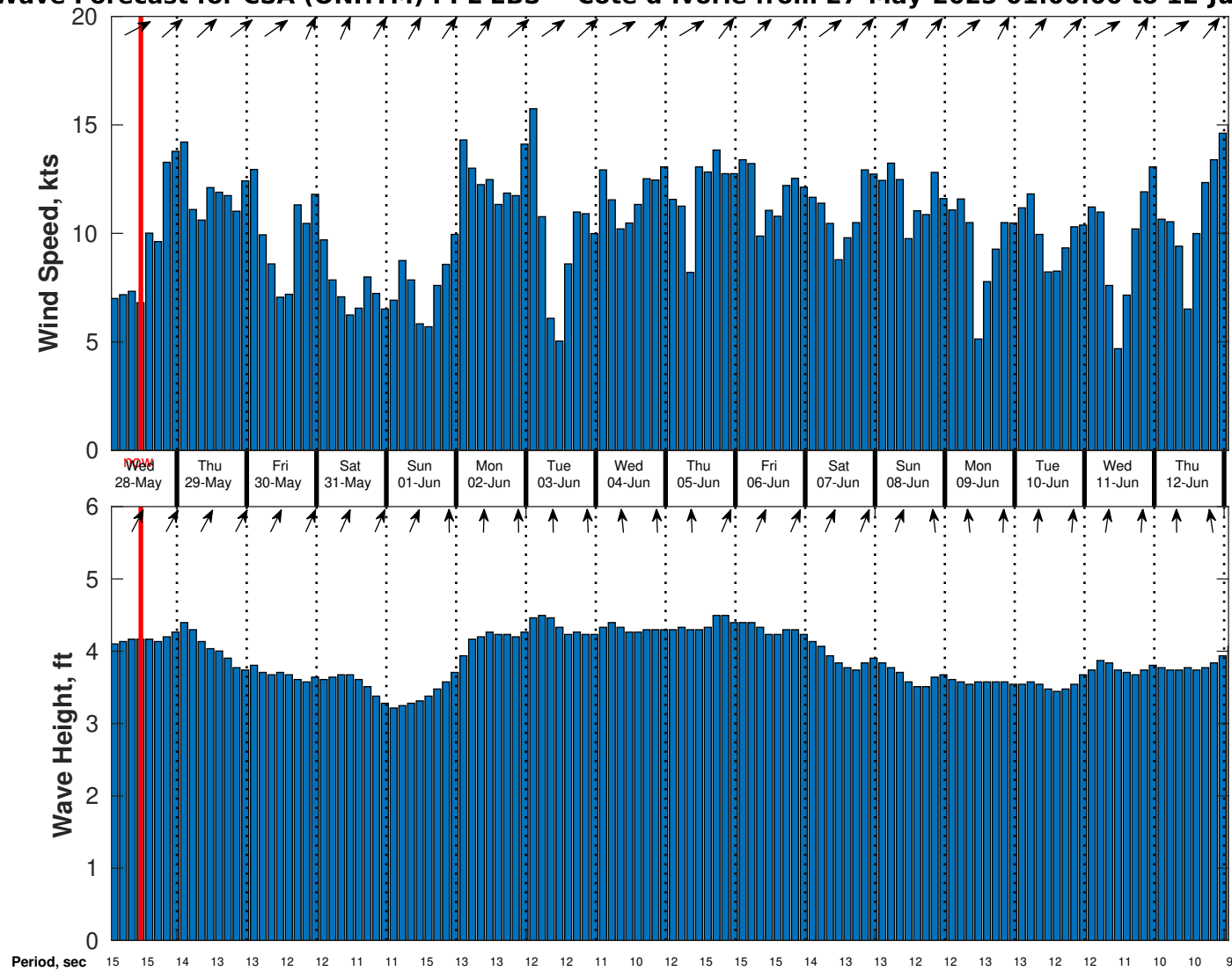
Wind & Wave Forecast for CSA (ONHYM) PPL EBS - Cote d'Ivoire from 27-May-2025 01:00:00 to 12-Jun-2025 01:00:00
