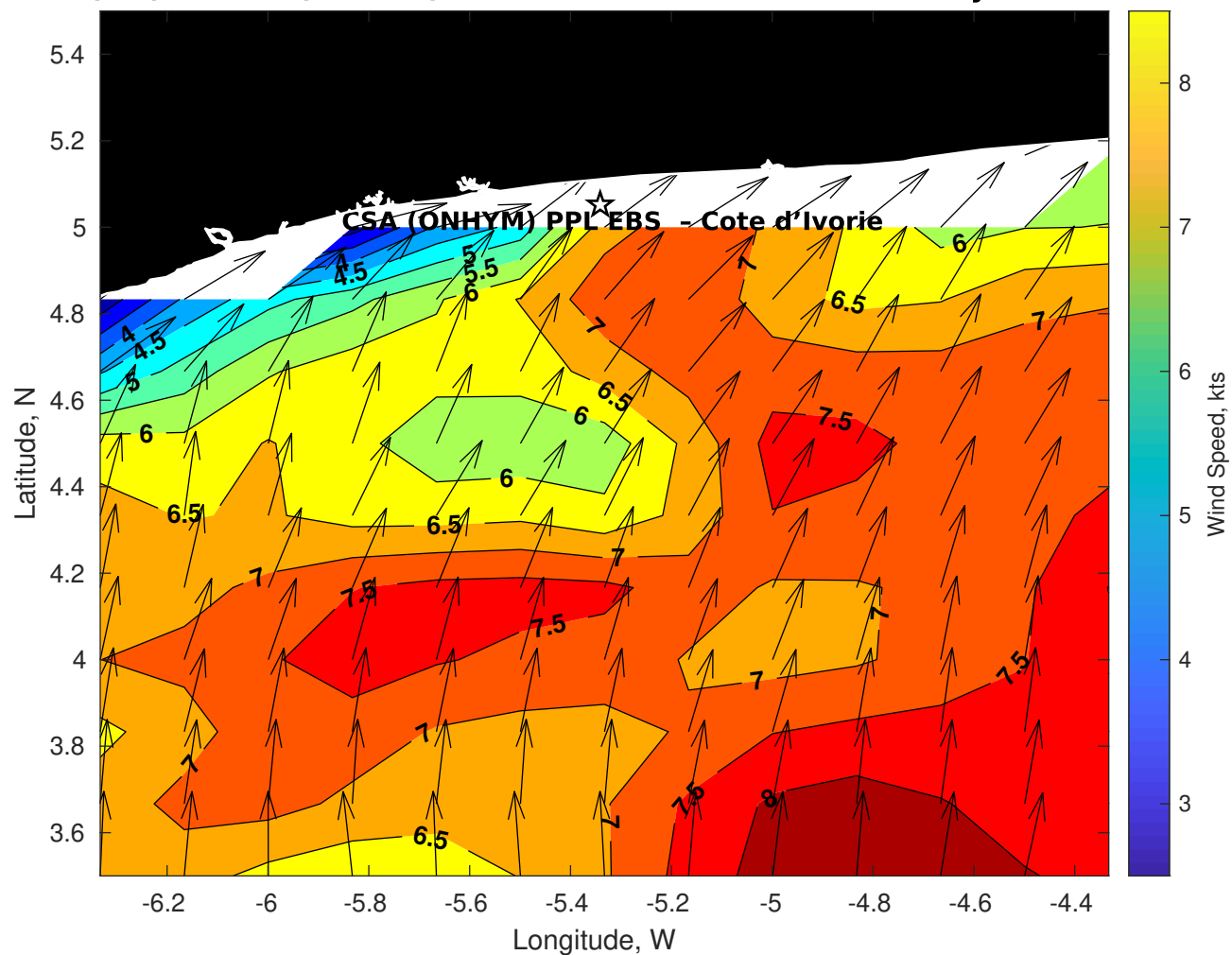
Winds (kts) for CSA (ONHYM) PPL EBS - Cote d'Ivoire at 27-May-2025 09:00:00
