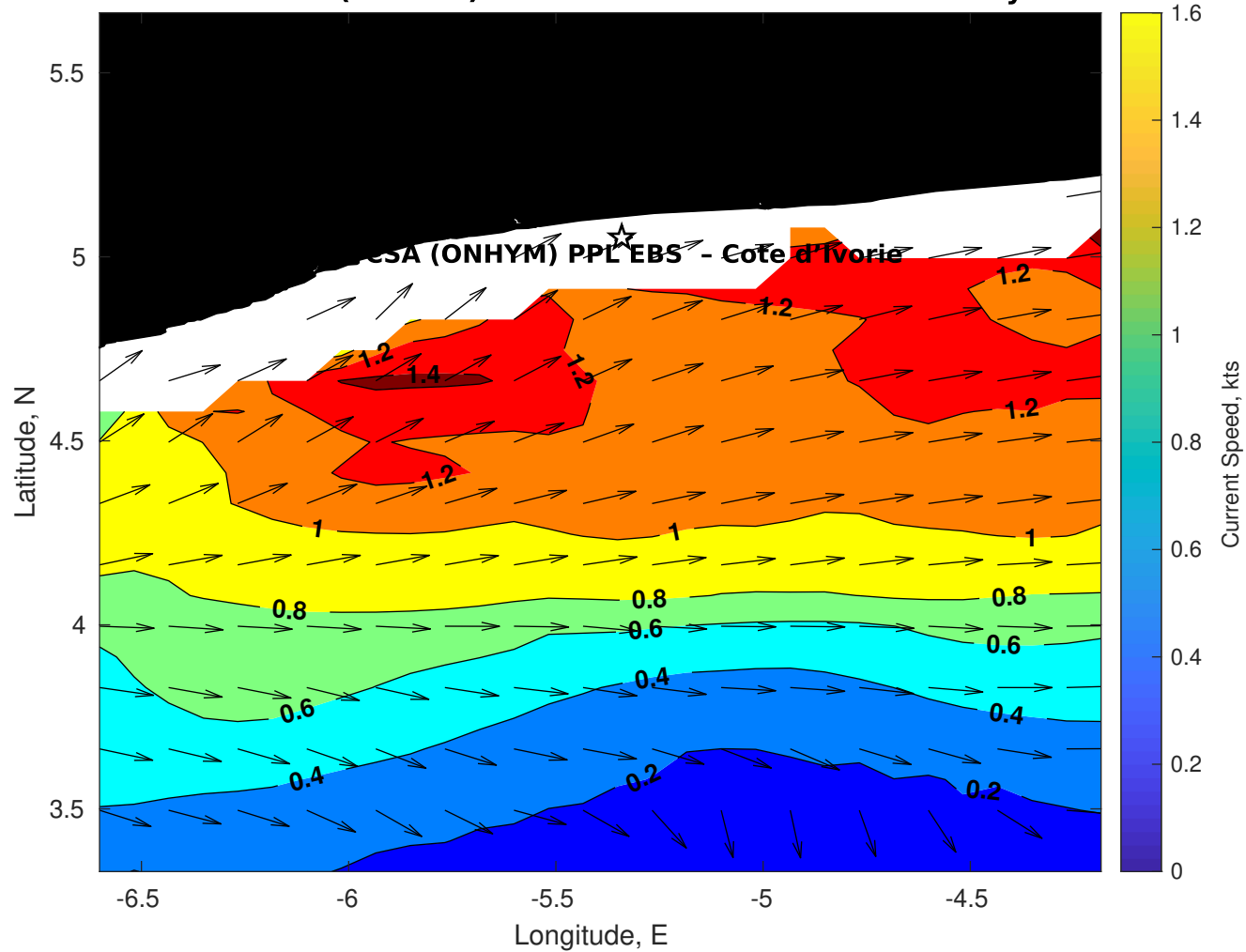
Surface Currents for CSA (ONHYM) PPL EBS - Cote d'Ivoire at 26-May-2025 00:00:00
