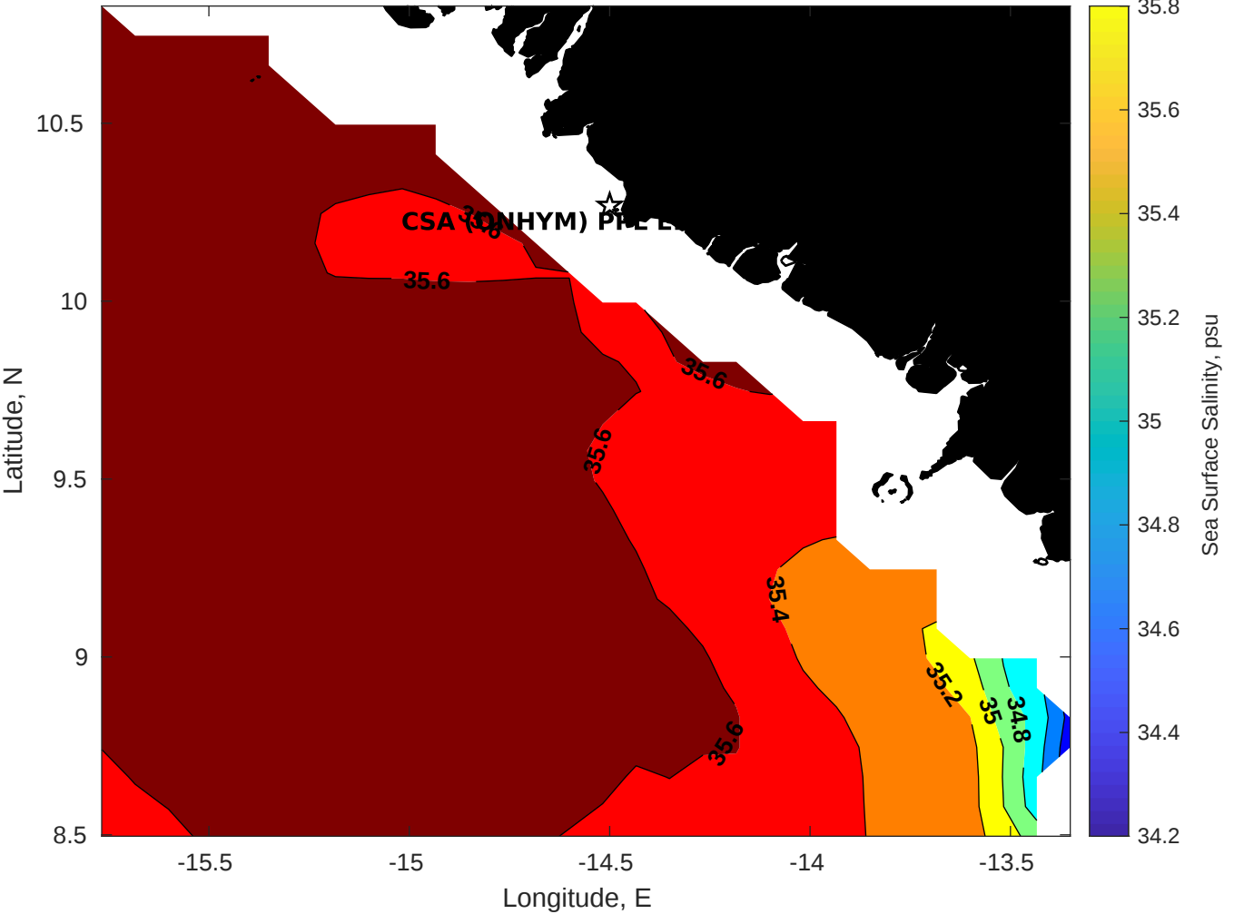
Surface Salinity for CSA (ONHYM) PPL EBS - Guinea at 26-May-2025 00:00:00
