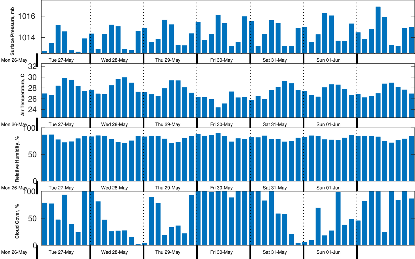
Met Forecast for CSA (ONHYM) PPL EBS - Liberia from 27-May-2025 00:00:00 to 03-Jun-2025 00:00:00
