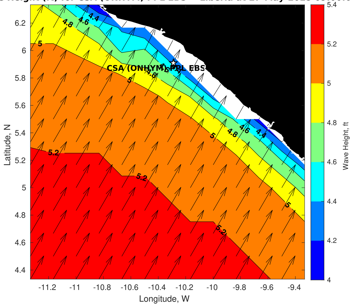
Wave Height (ft) for CSA (ONHYM) PPL EBS - Liberia at 27-May-2025 09:00:00
