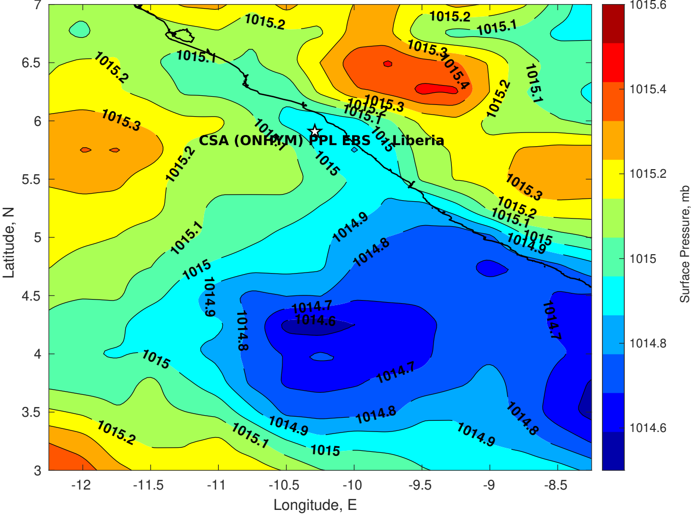
Surface Pressure (mb) for CSA (ONHYM) PPL EBS - Liberia at 29-May-2025 00:00:00
