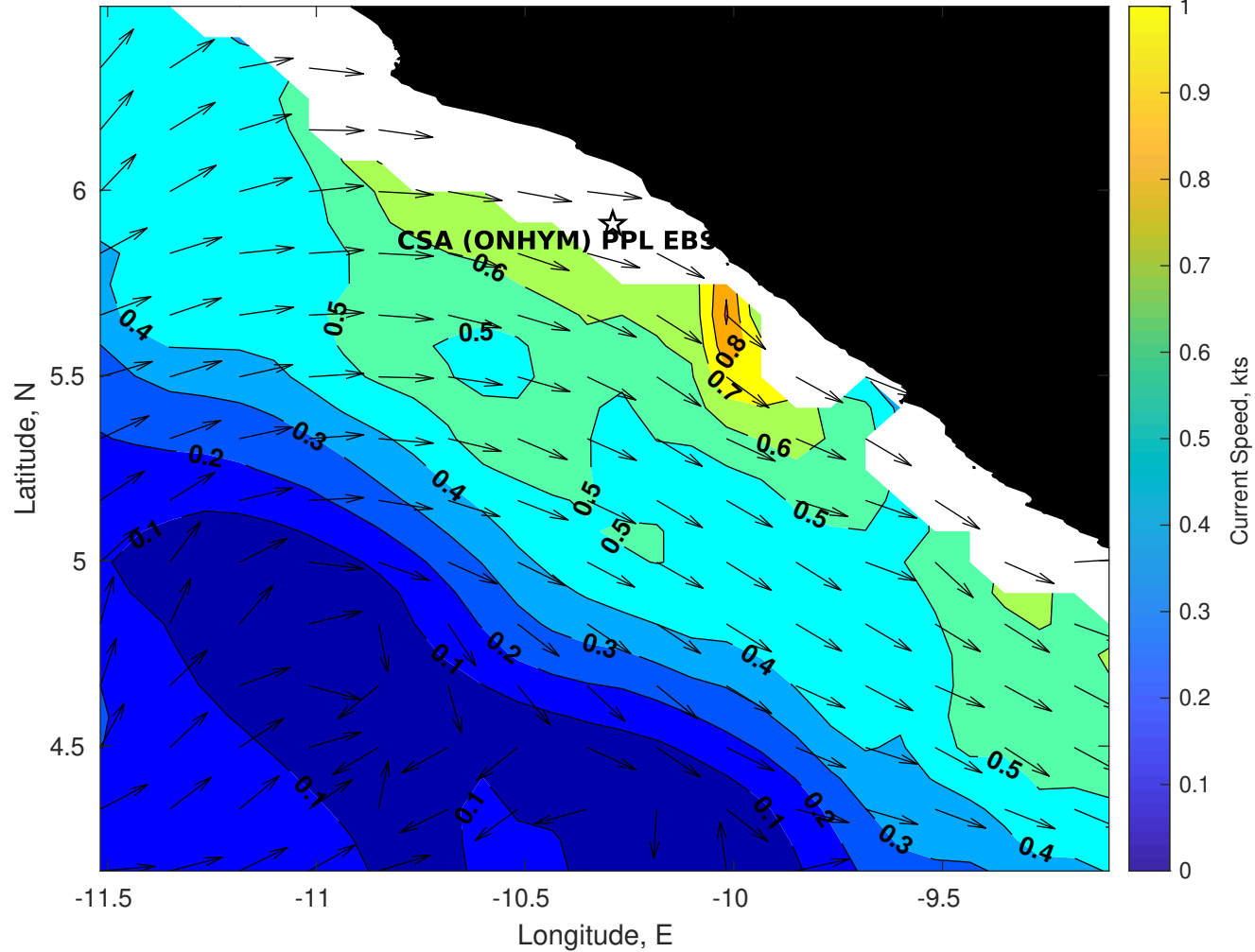
Surface Currents for CSA (ONHYM) PPL EBS - Liberia at 26-May-2025 00:00:00
