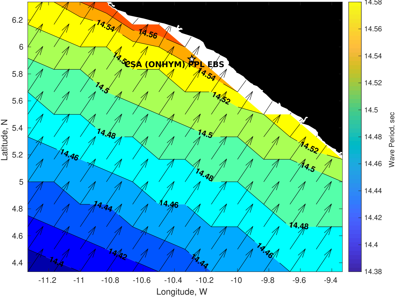
Wave Period (sec) for CSA (ONHYM) PPL EBS - Liberia at 27-May-2025 09:00:00
