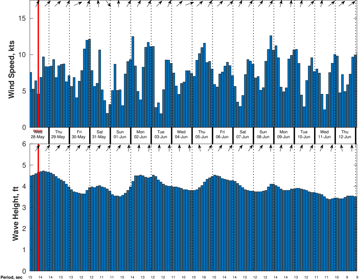
Wind & Wave Forecast for CSA (ONHYM) PPL EBS - Liberia from 27-May-2025 01:00:00 to 12-Jun-2025 01:00:00
