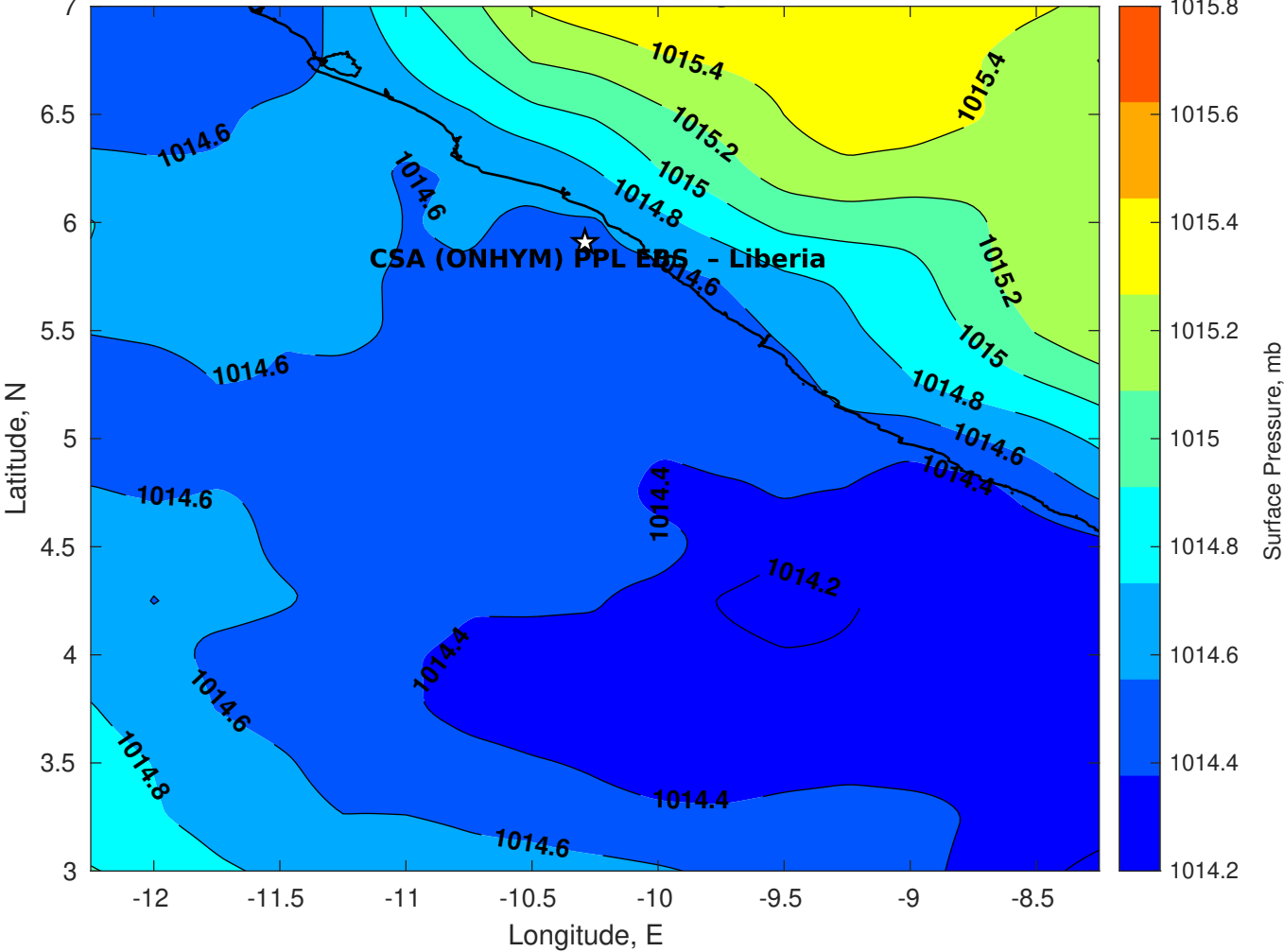
Surface Pressure (mb) for CSA (ONHYM) PPL EBS - Liberia at 27-May-2025 00:00:00
