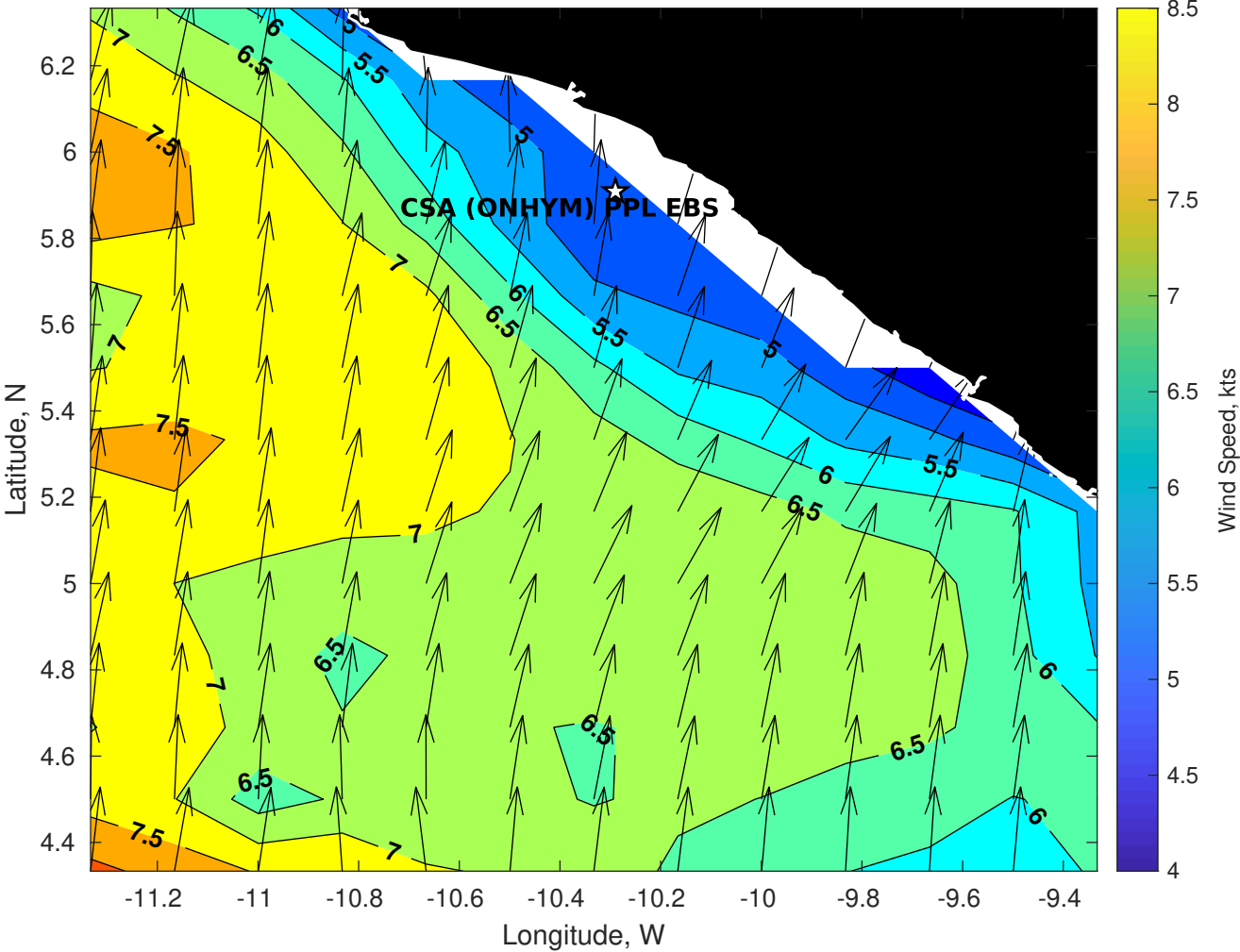
Winds (kts) for CSA (ONHYM) PPL EBS - Liberia at 27-May-2025 09:00:00
