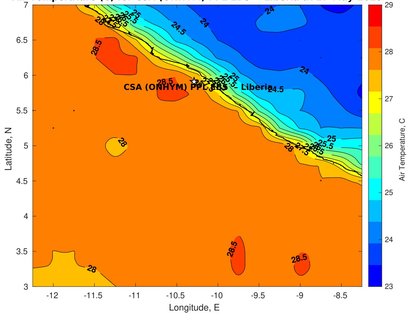
Air Temperature (C) for CSA (ONHYM) PPL EBS - Liberia at 27-May-2025
