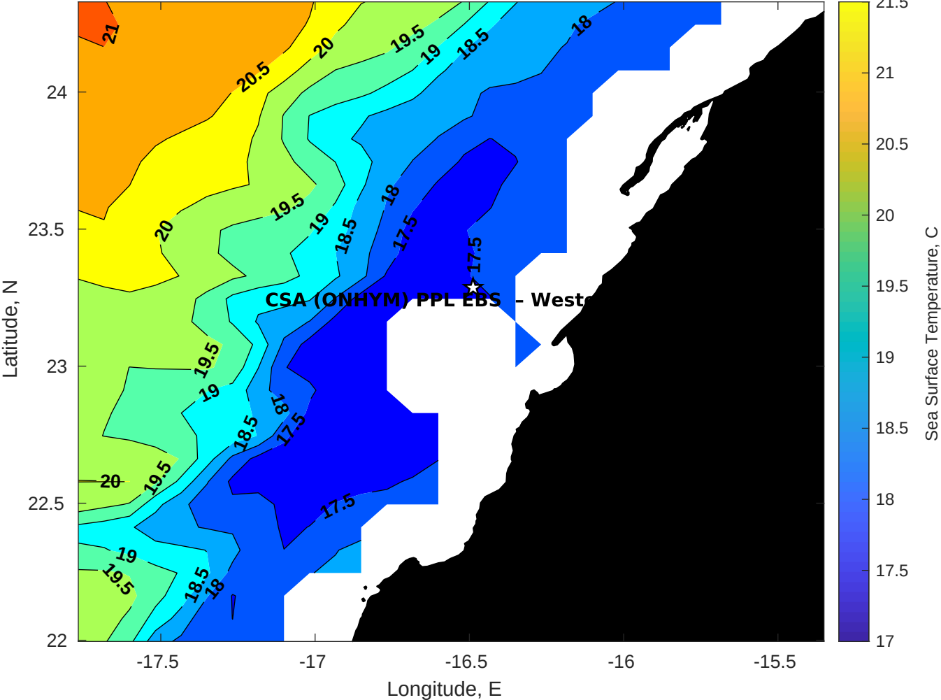
SST for CSA (ONHYM) PPL EBS - Western Sahara at 26-May-2025 00:00:00
