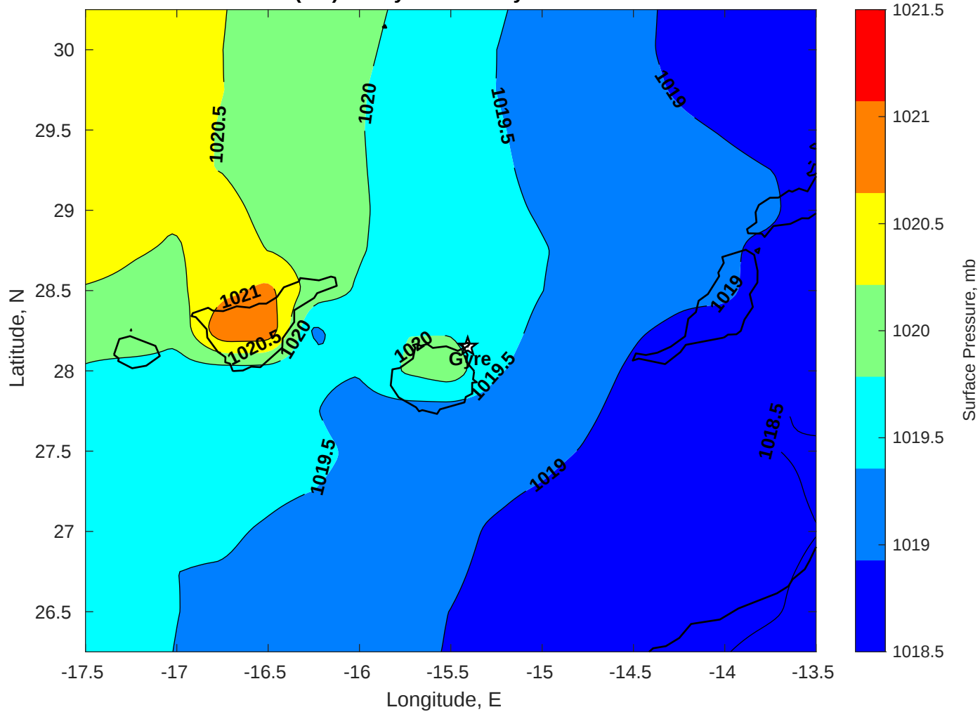
Surface Pressure (mb) for Gyre at 30-May-2025 00:00:00
