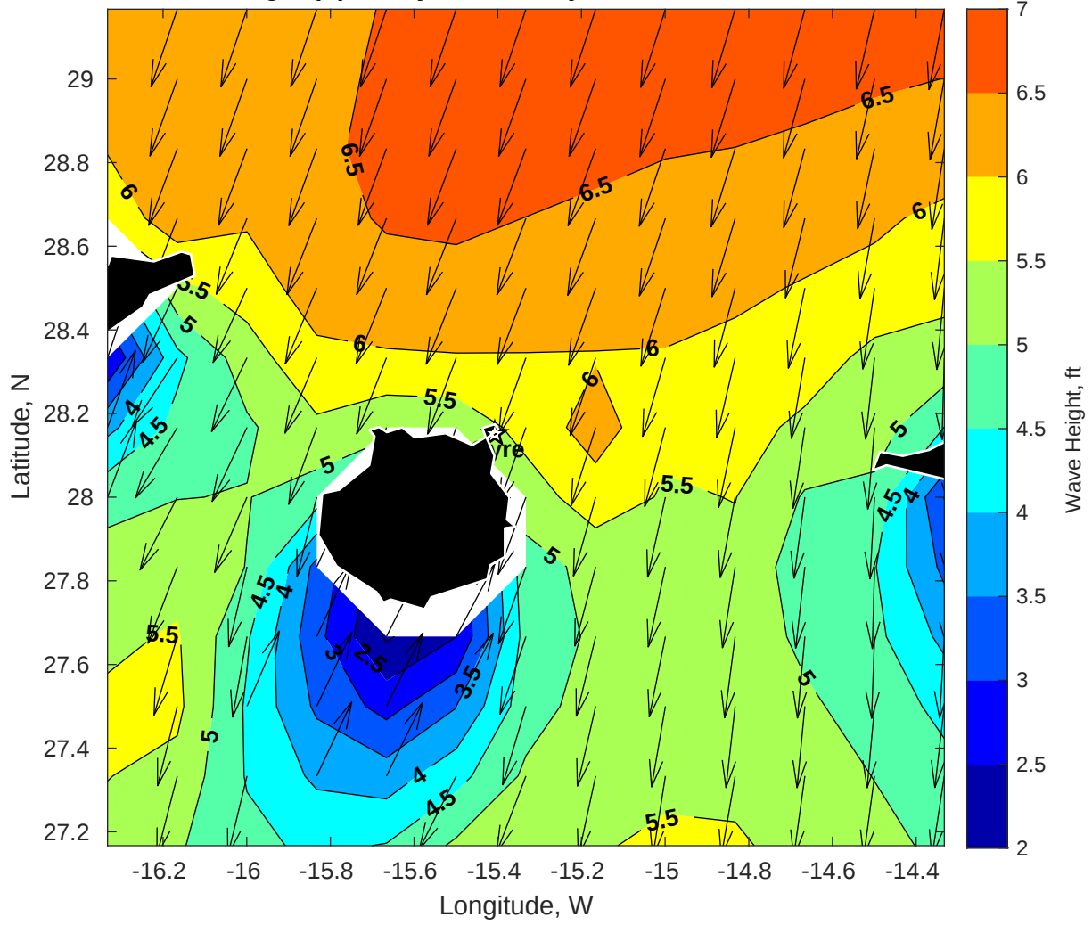
Wave Height (ft) for Gyre at 28-May-2025 09:00:00
