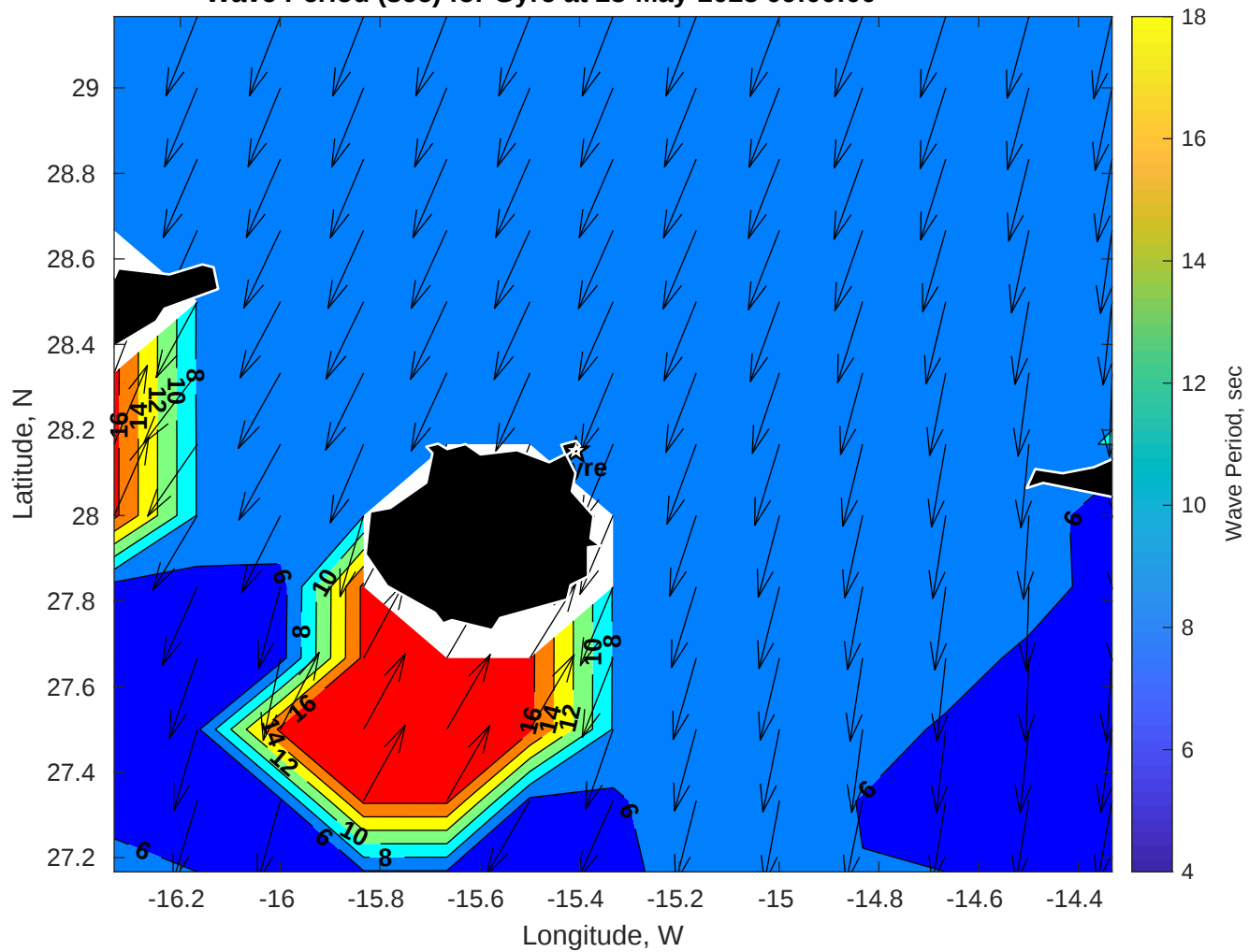
Wave Period (sec) for Gyre at 28-May-2025 09:00:00
