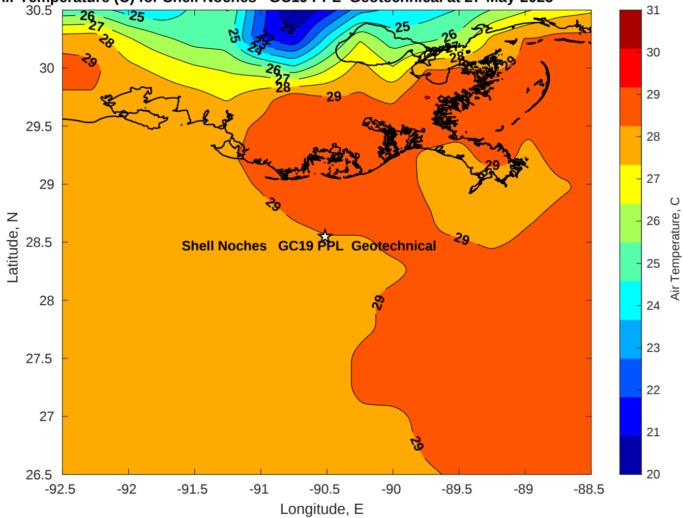
Air Temperature (C) for Shell Noches GC19 PPL Geotechnical at 27-May-2025
