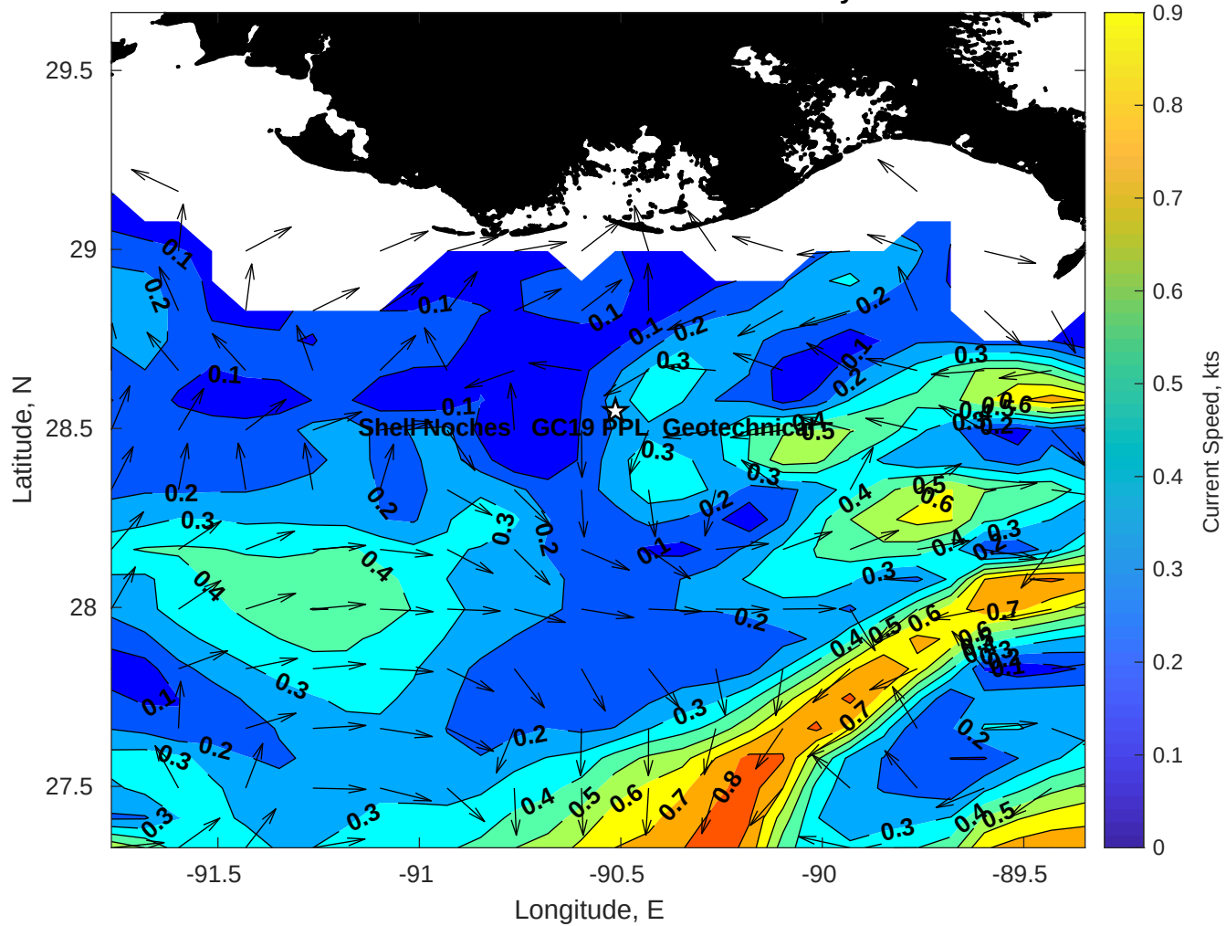
Surface Currents for Shell Noches GC19 PPL Geotechnical at 26-May-2025 00:00:00
