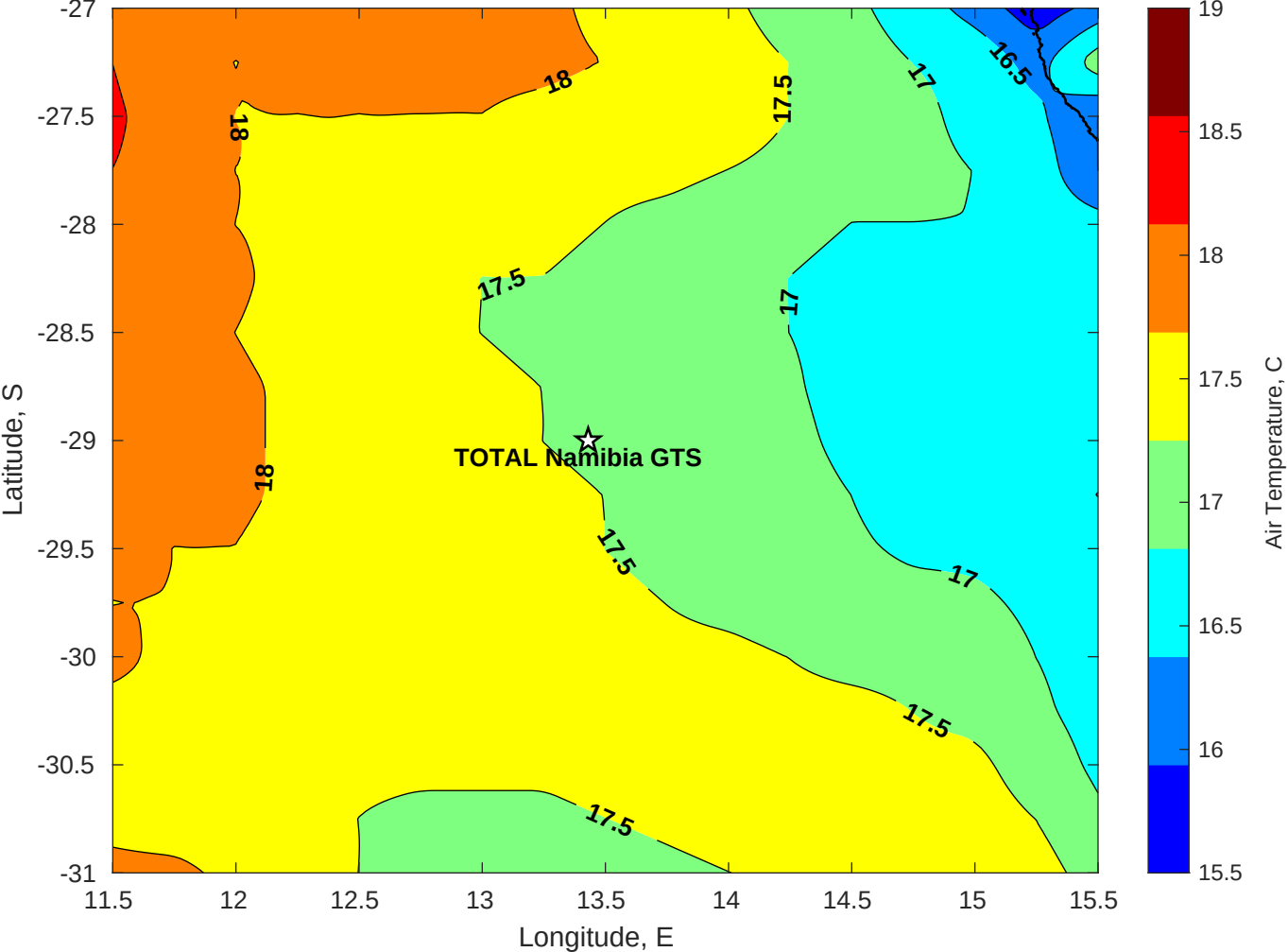
Air Temperature (C) for TOTAL Namibia GTS at 27-May-2025
