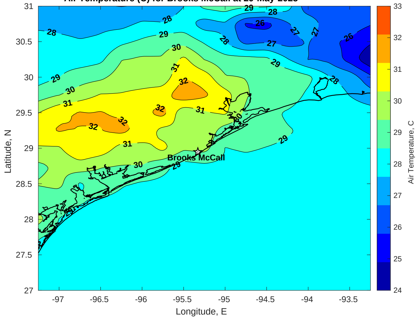
Air Temperature (C) for Brooks McCall at 29-May-2025
