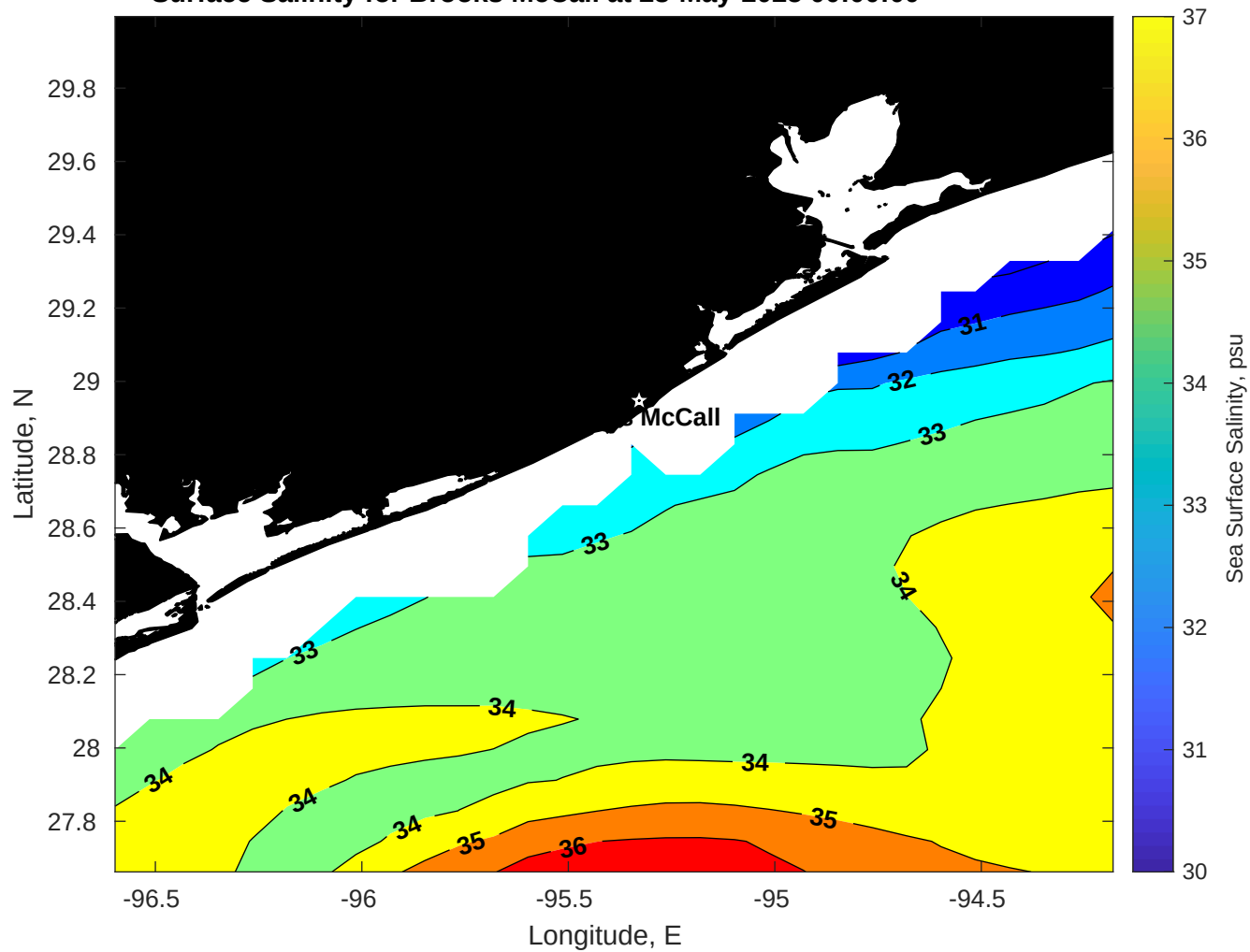
Surface Salinity for Brooks McCall at 28-May-2025 00:00:00
