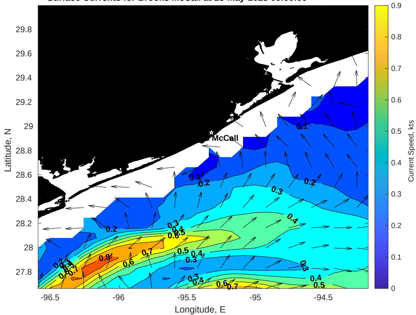
Surface Currents for Brooks McCall at 28-May-2025 00:00:00
