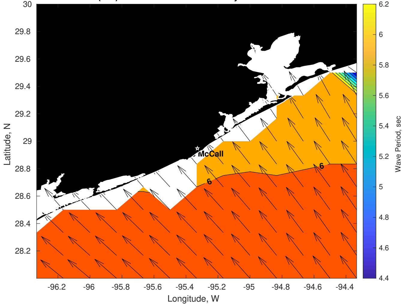
Wave Period (sec) for Brooks McCall at 29-May-2025 09:00:00
