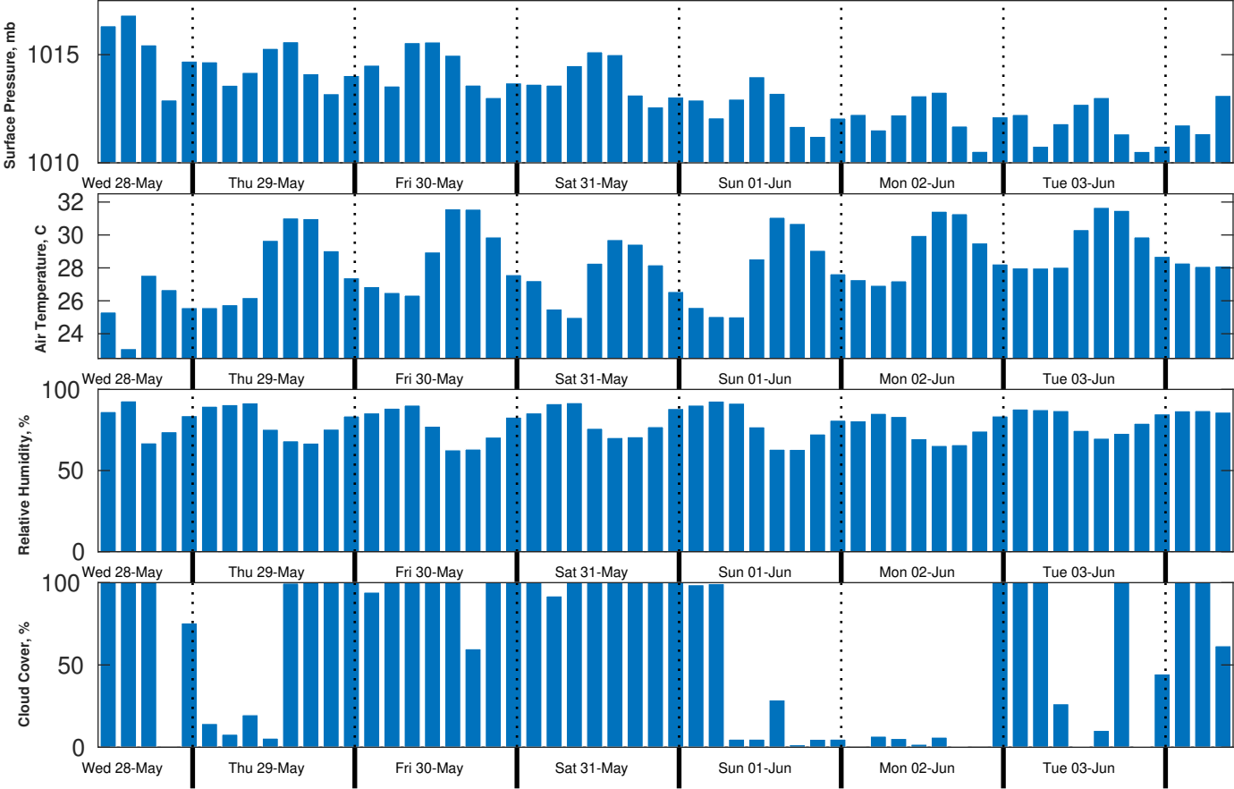
Met Forecast for Brooks McCall from 28-May-2025 12:00:00 to 04-Jun-2025 12:00:00
