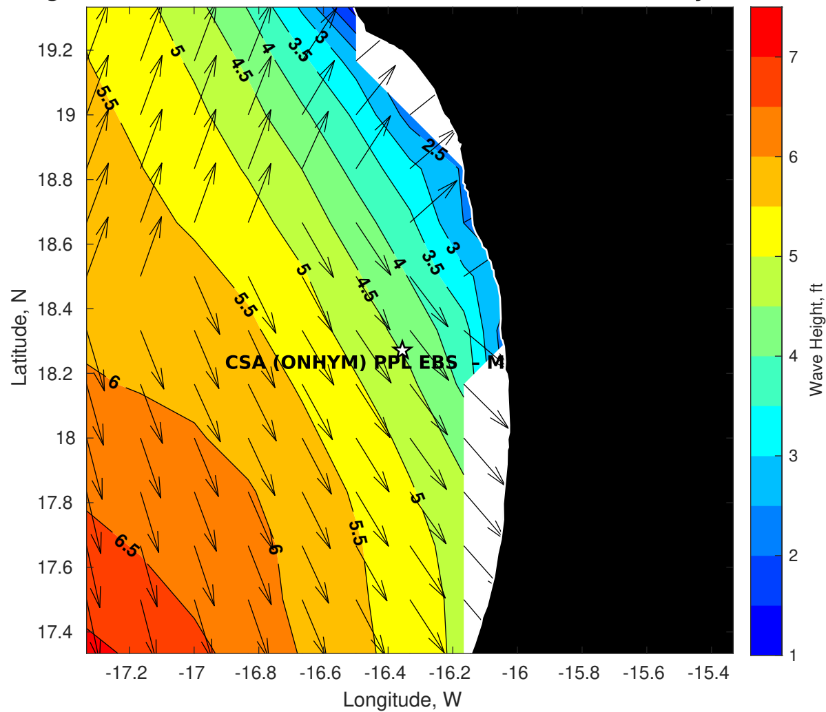
Wave Height (ft) for CSA (ONHYM) PPL EBS - Mauritania at 27-May-2025 09:00:00
