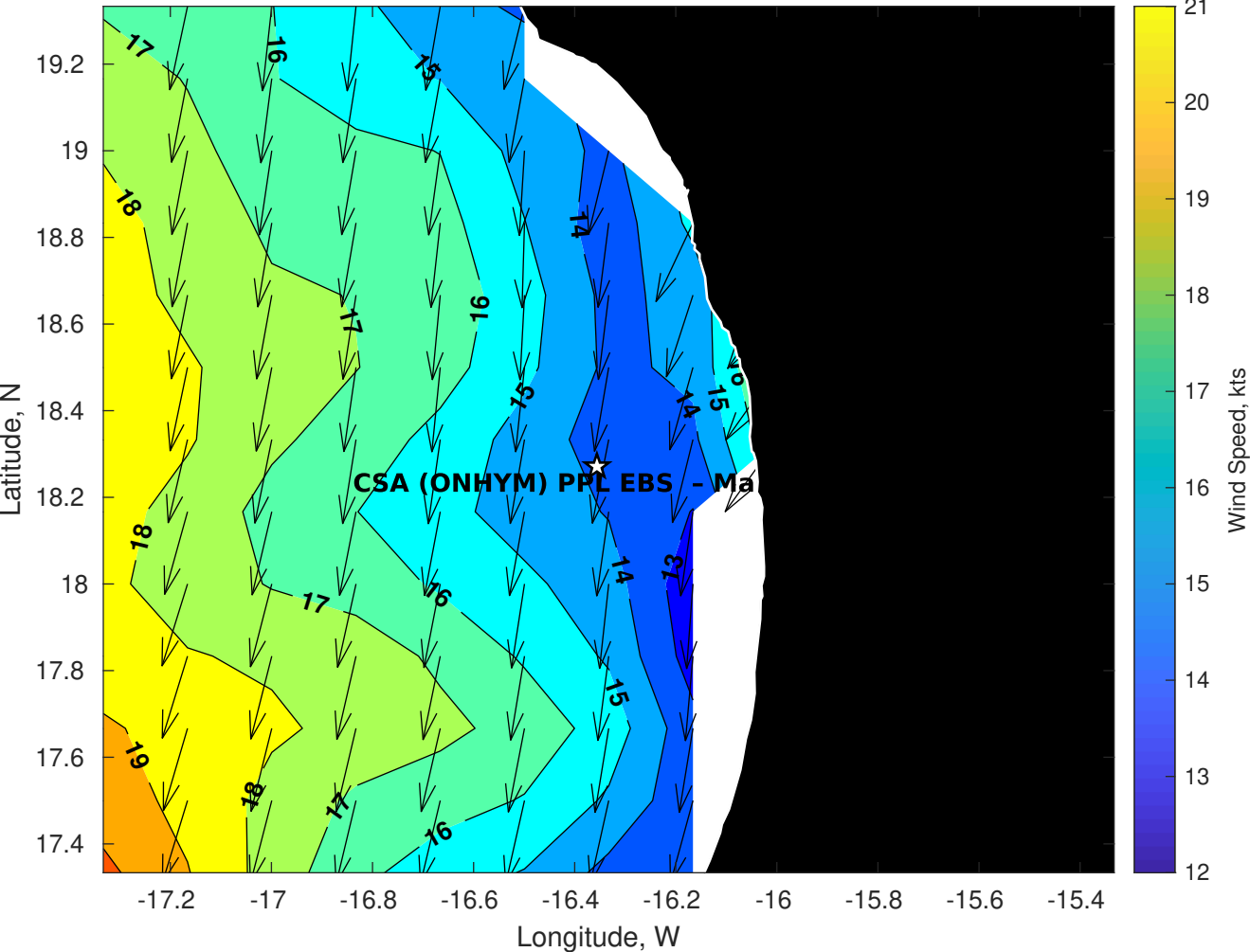
Winds (kts) for CSA (ONHYM) PPL EBS - Mauritania at 27-May-2025 09:00:00
