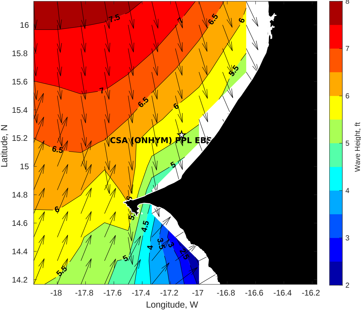
Wave Height (ft) for CSA (ONHYM) PPL EBS - Senegal at 27-May-2025 09:00:00
